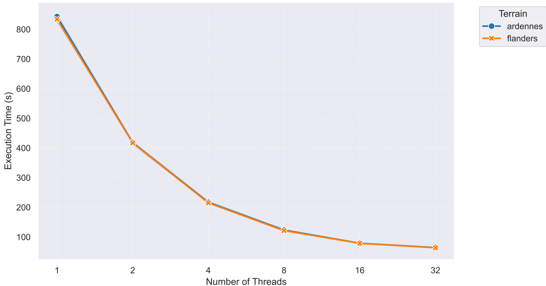
Execution Time vs Threads (95% CI) Constants: Mutation Prob = 0.15 | Population = 1000 | Sensors = 100 | Generations = 100 | Grid Size = 200x200
