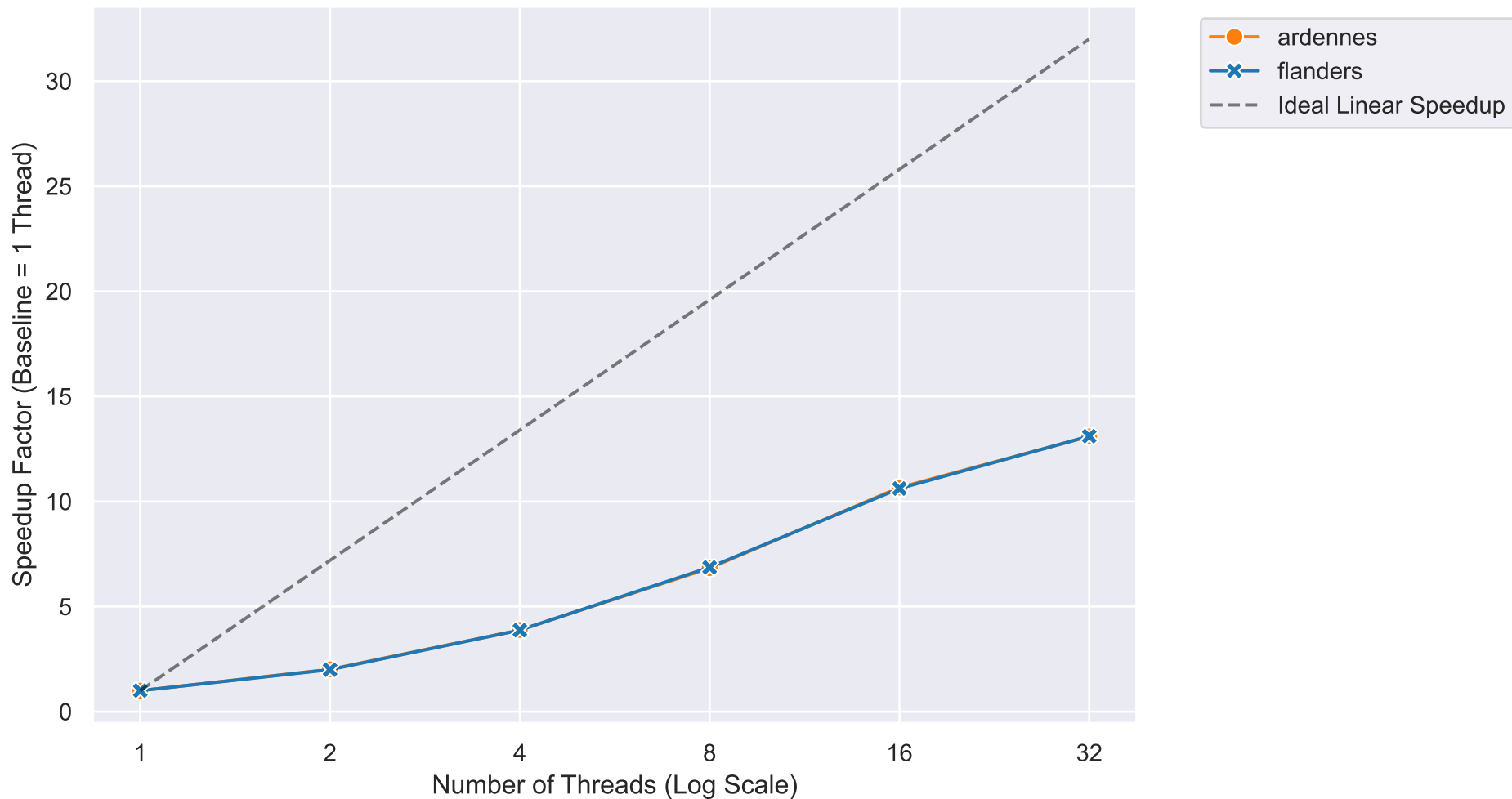
Speedup vs Number of Threads Constants: Mutation Prob = 0.15 | Population = 1000 | Sensors = 100 | Generations = 100 | Grid Size = 200x200
