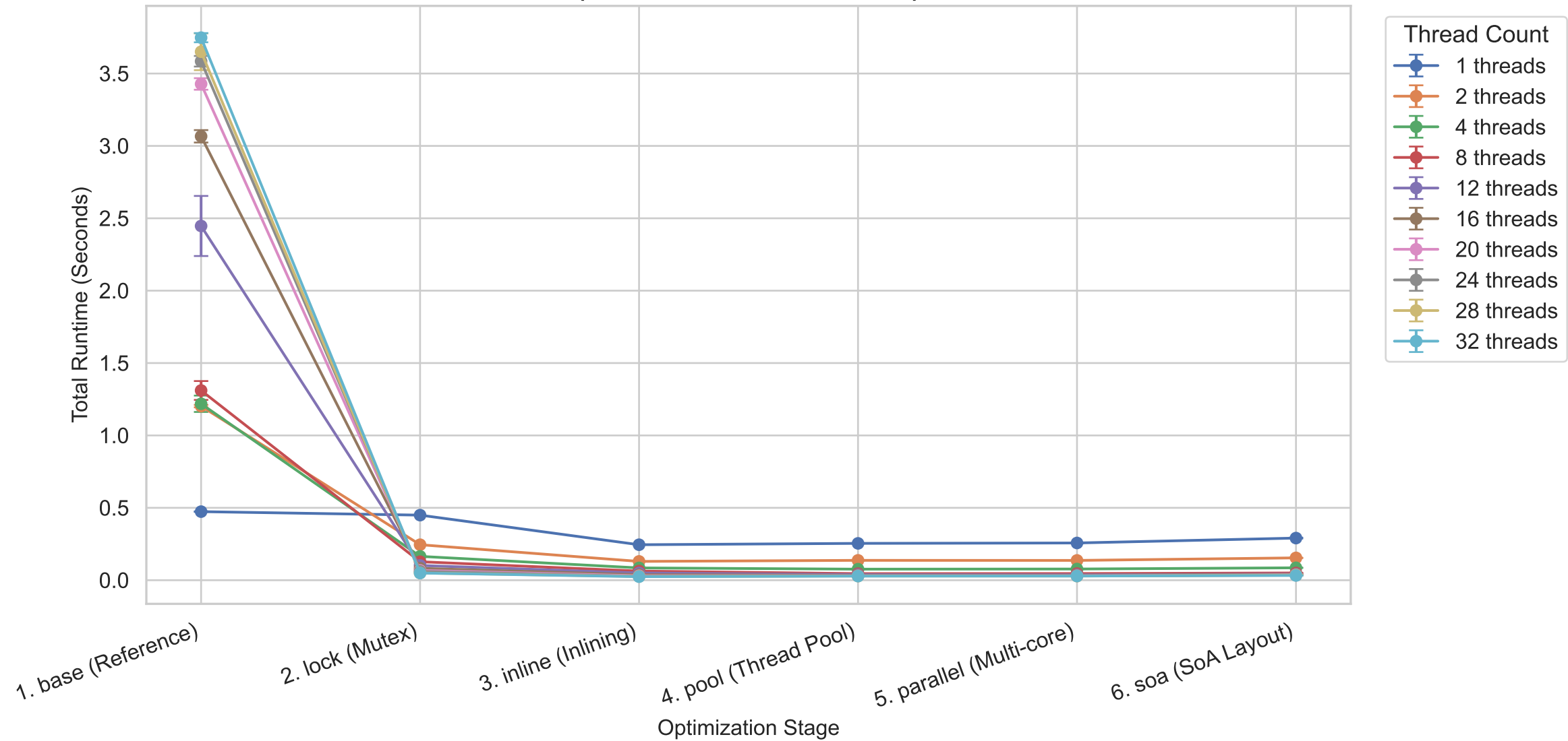
Total Time Performance Progression — Scene: Box (95% Confidence Intervals)
