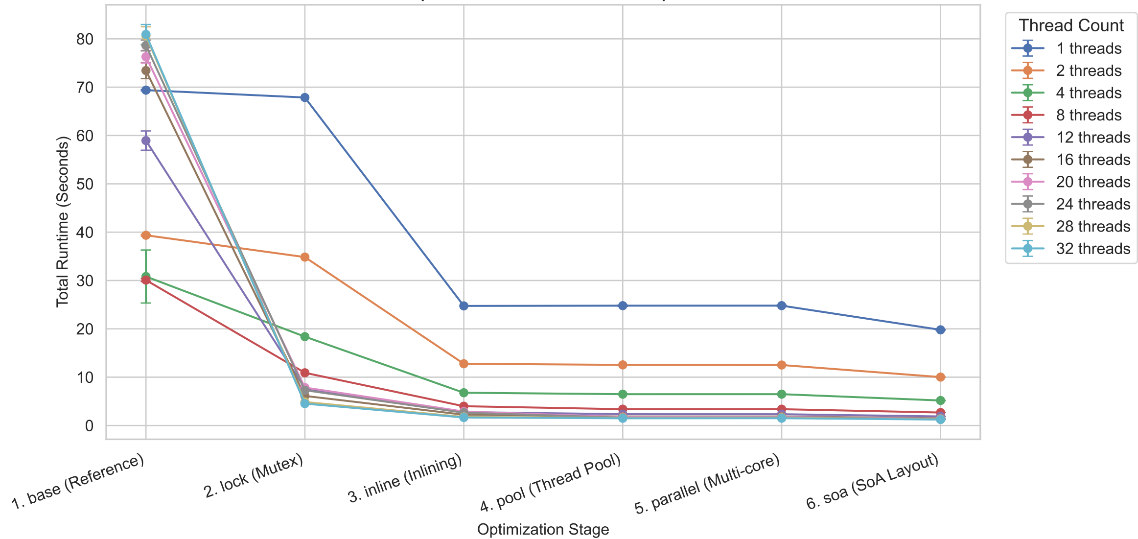
Total Time Performance Progression — Scene: Cornell-Box (95% Confidence Intervals)
