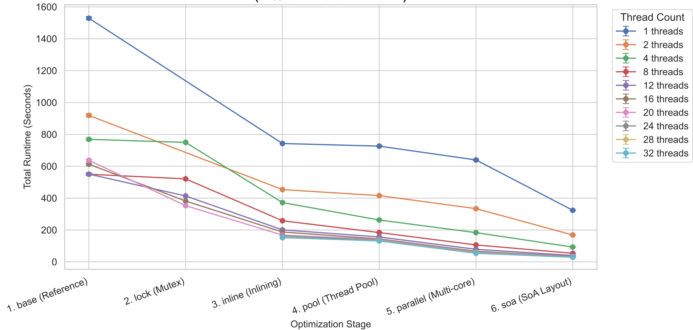
Total Time Performance Progression — Scene: Dragon (95% Confidence Intervals)
