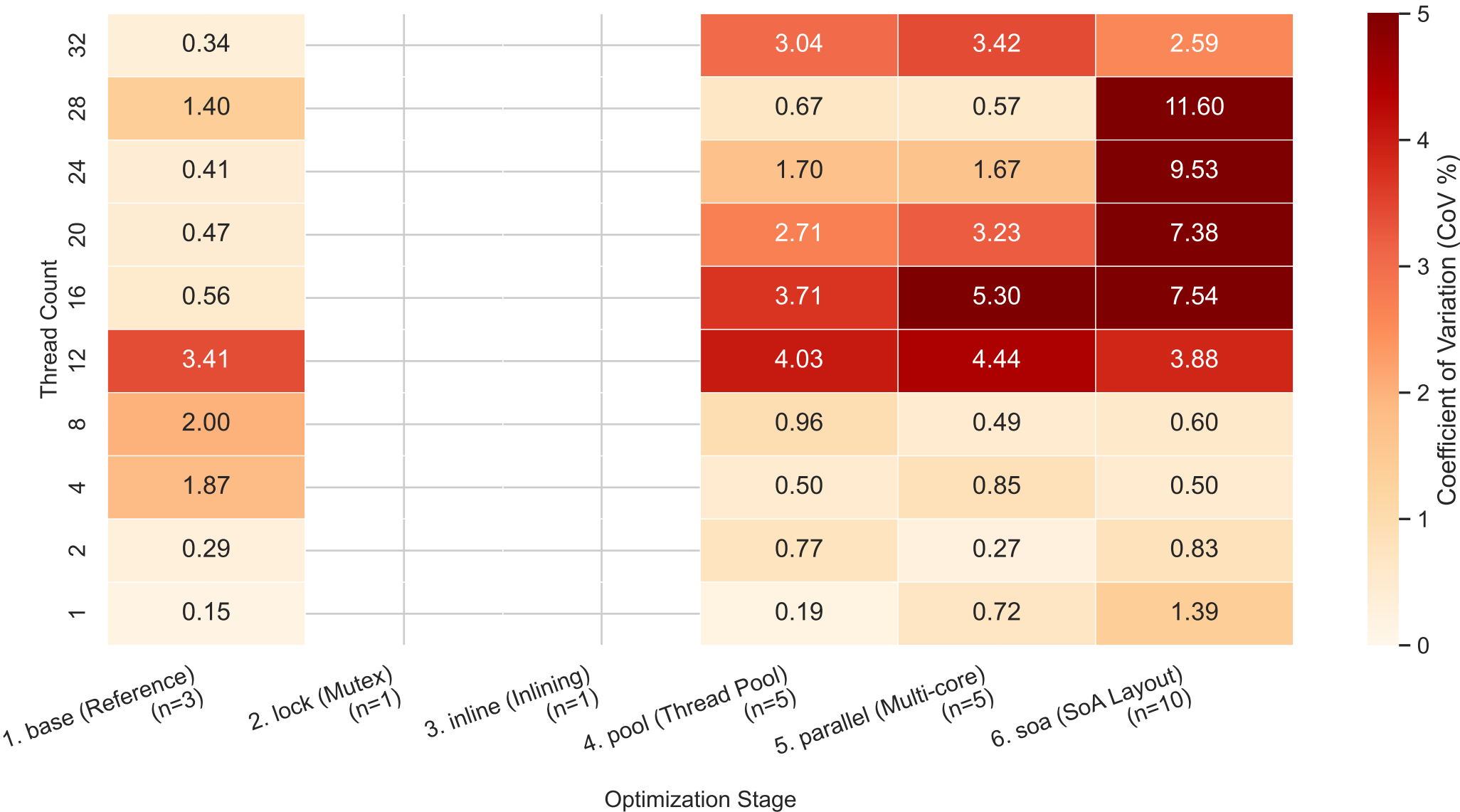
Benchmark Run Stability Heatmap (CoV%) — Scene: Box (CoV Range: 0% - 5%)
