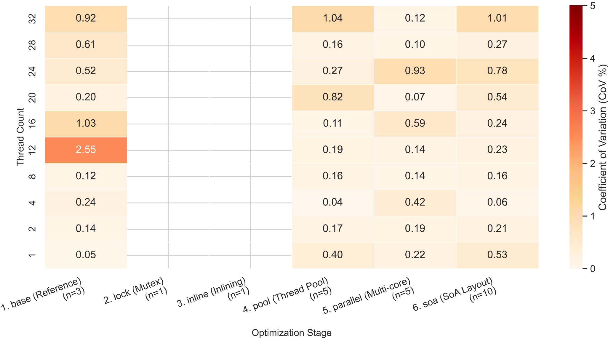
Benchmark Run Stability Heatmap (CoV%) — Scene: Cornell-Spheres (CoV Range: 0% - 5%)
