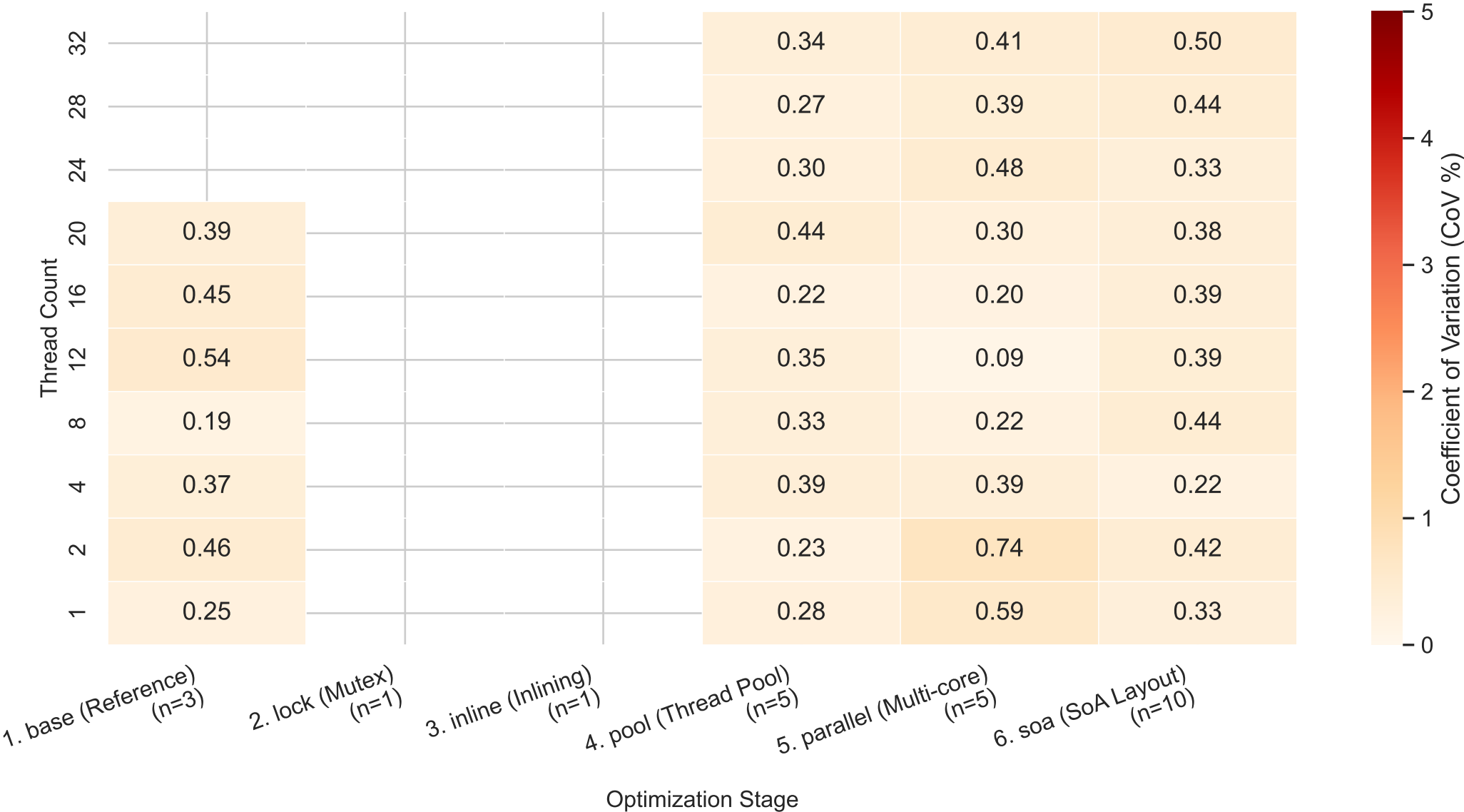
Benchmark Run Stability Heatmap (CoV%) — Scene: Dragon (CoV Range: 0% - 5%)
