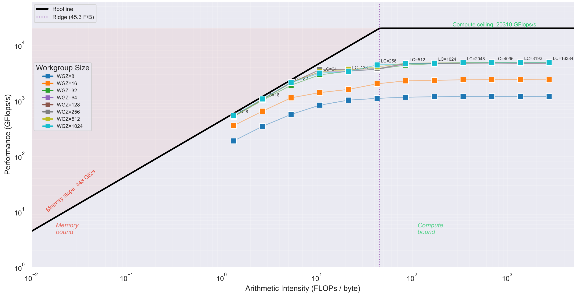
Roofline Model — [add] — All Workgroup Sizes
