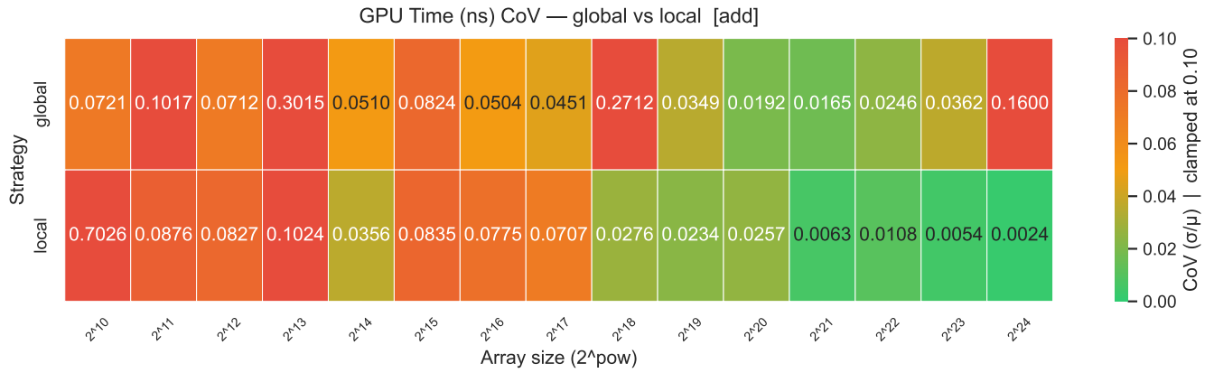
Figure 31: Desktop - Part 4 - GPU Time CoV
