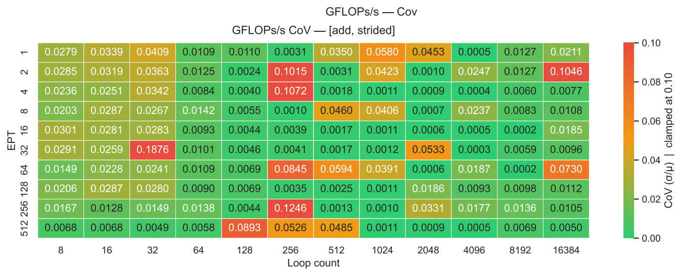
Figure 27: Desktop - Part 3 - Compute Throughput CoV
