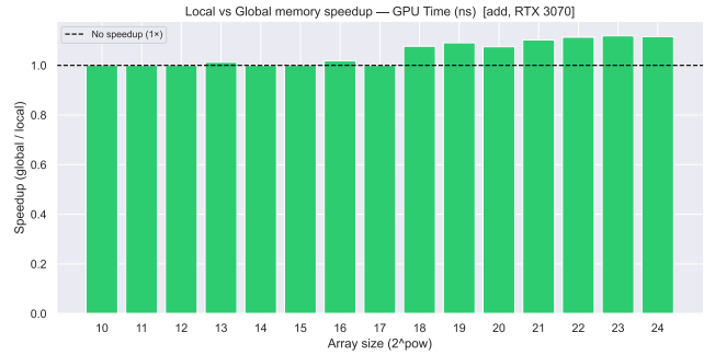
Figure 18: Local vs Global Speedup
