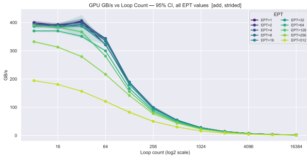
Figure 13: Memory Bandwidth Utilization vs Loop Count
