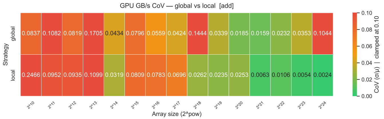
Figure 32: Desktop - Part 4 - Memory Bandwidth CoV
