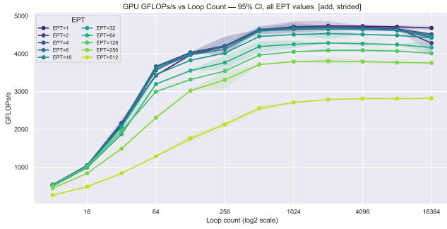
Figure 12: GPU Compute Throughput vs Loop Count
