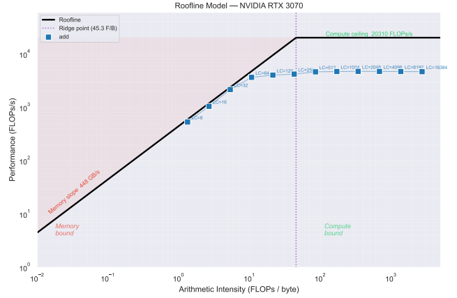
Figure 14: RTX3070 - Roofline Model
