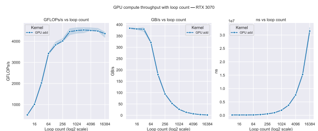
Figure 11: Loop Count vs Compute; Bandwidth & Execution Time
