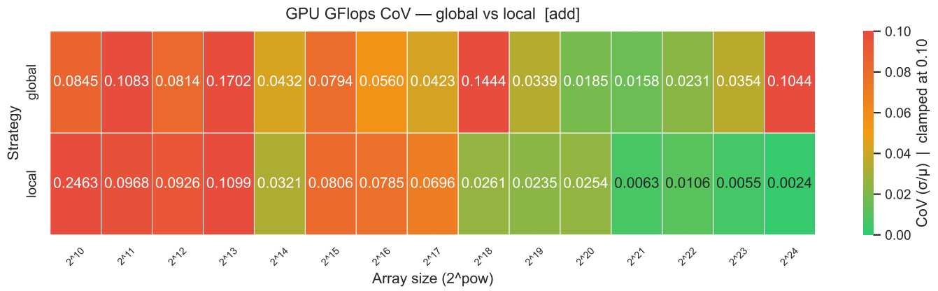
Figure 33: Desktop - Part 4 - Compute Throughput CoV
