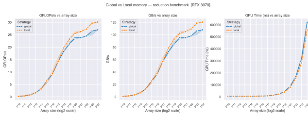
Figure 17: Global vs Local - GPU Time, Compute & Memory Bandwidth
