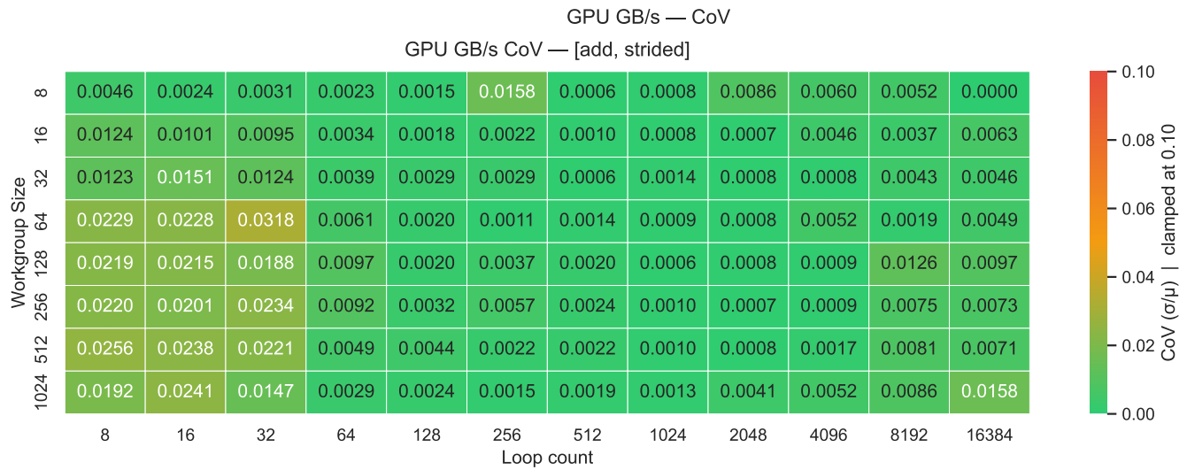
Figure 29: Desktop - Part 3.2 - Memory Bandwidth CoV
