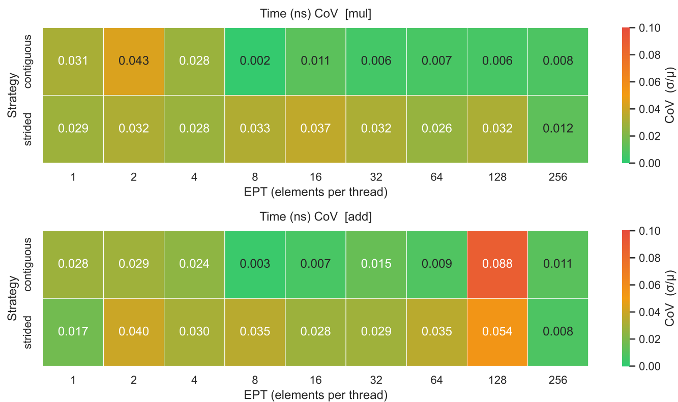
Figure 24: Desktop - Part 2 - GPU Time CoV
