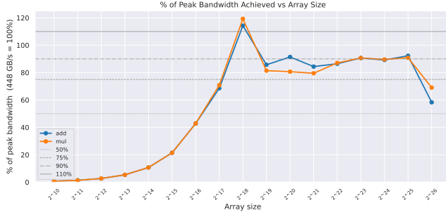
Figure 4: Bandwidth Percentage Utilization vs Array Size
