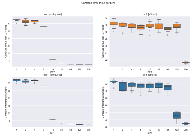
Figure 10: Computational Throughput CI Intervals
