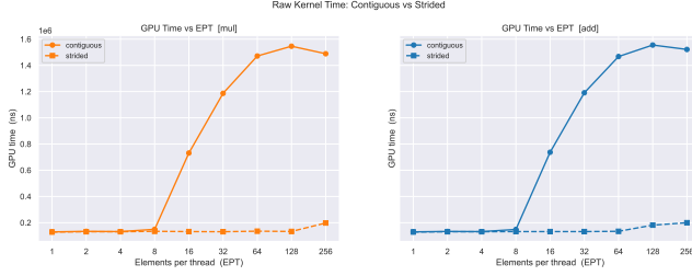
Figure 7: GPU Execution Time vs EPT - mul & add operations - contiguous vs strided pattern
