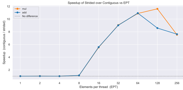
Figure 8: Strided Pattern Speedup vs Contiguous Pattern
