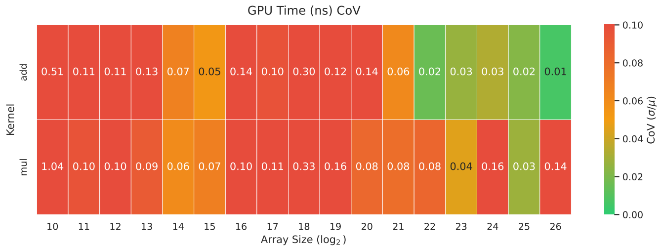
Figure 21: Desktop - Part 1 - GPU Time CoV
