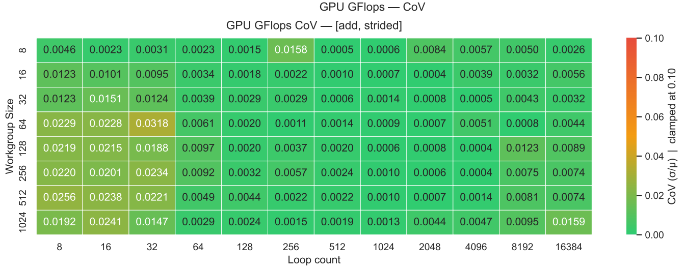
Figure 30: Desktop - Part 3.2 - Compute Throughput CoV
