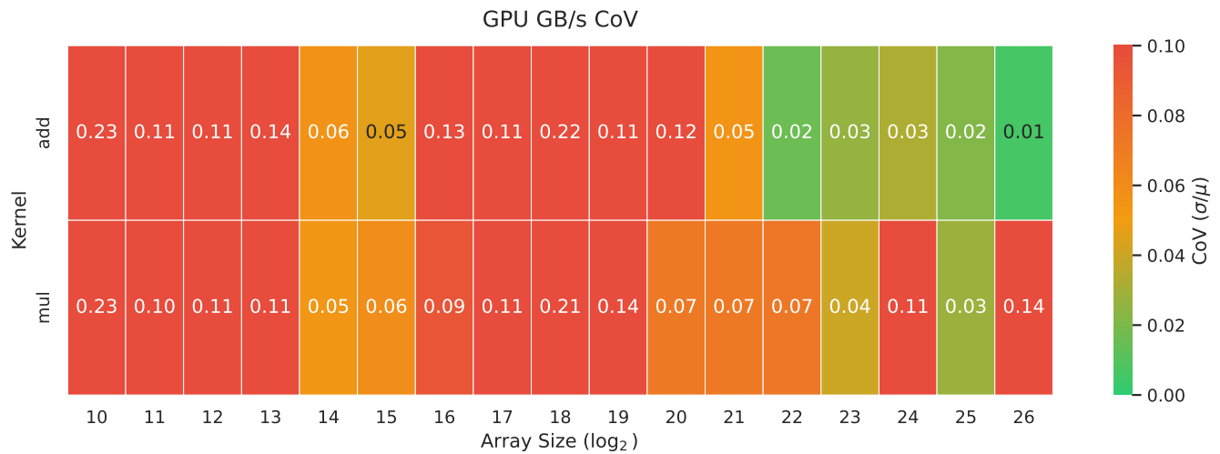
Figure 22: Desktop - Part 1 - Memory Bandwidth CoV
