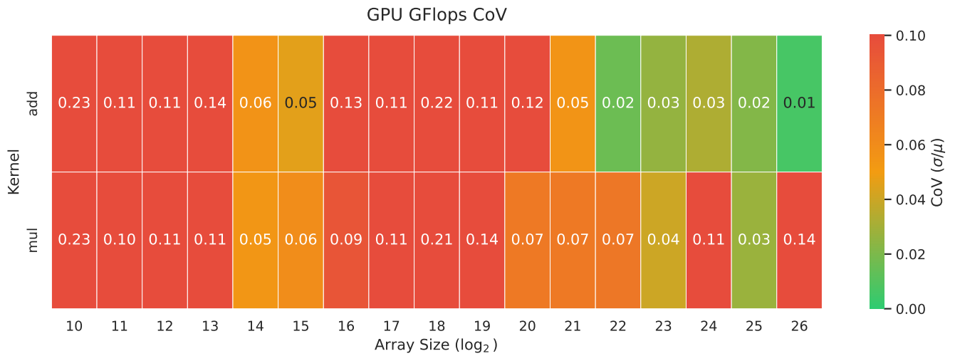
Figure 23: Desktop - Part 1 - Compute Throughput CoV
