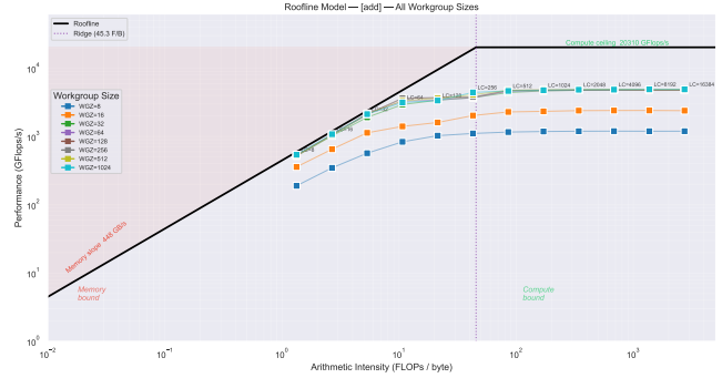
Figure 16: Roofline Model vs Workgroup Size
