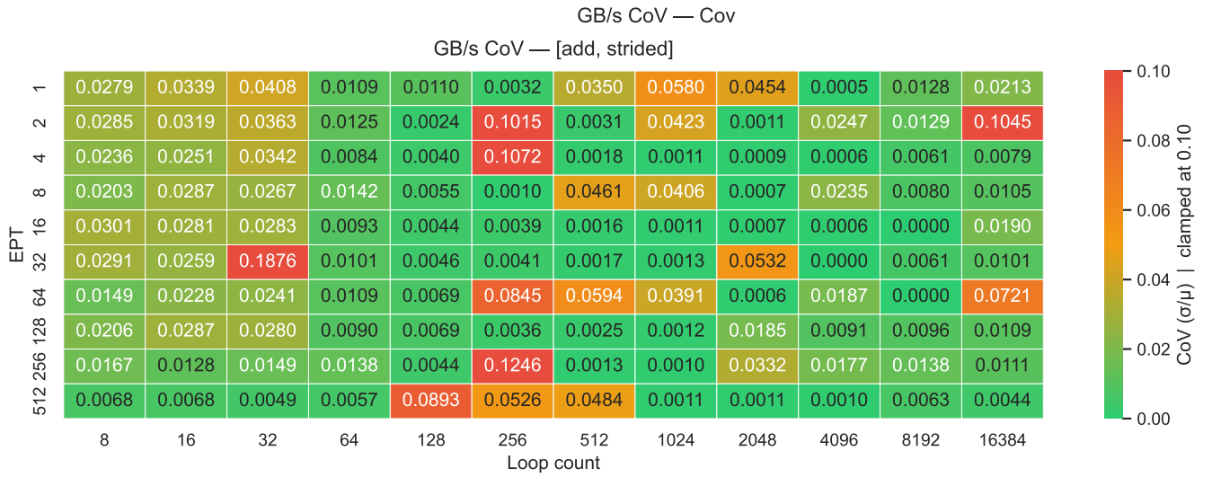
Figure 26: Desktop - Part “” - Memory Bandwidth CoV
