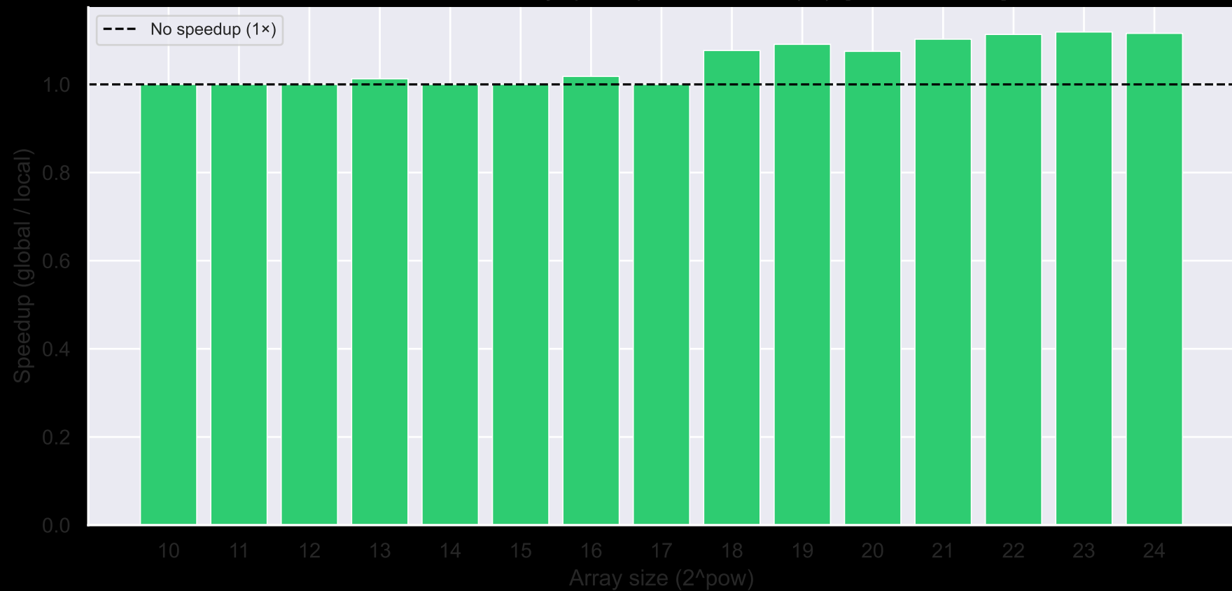
Local vs Global memory speedup — GPU Time (ns) [add, RTX 3070]
