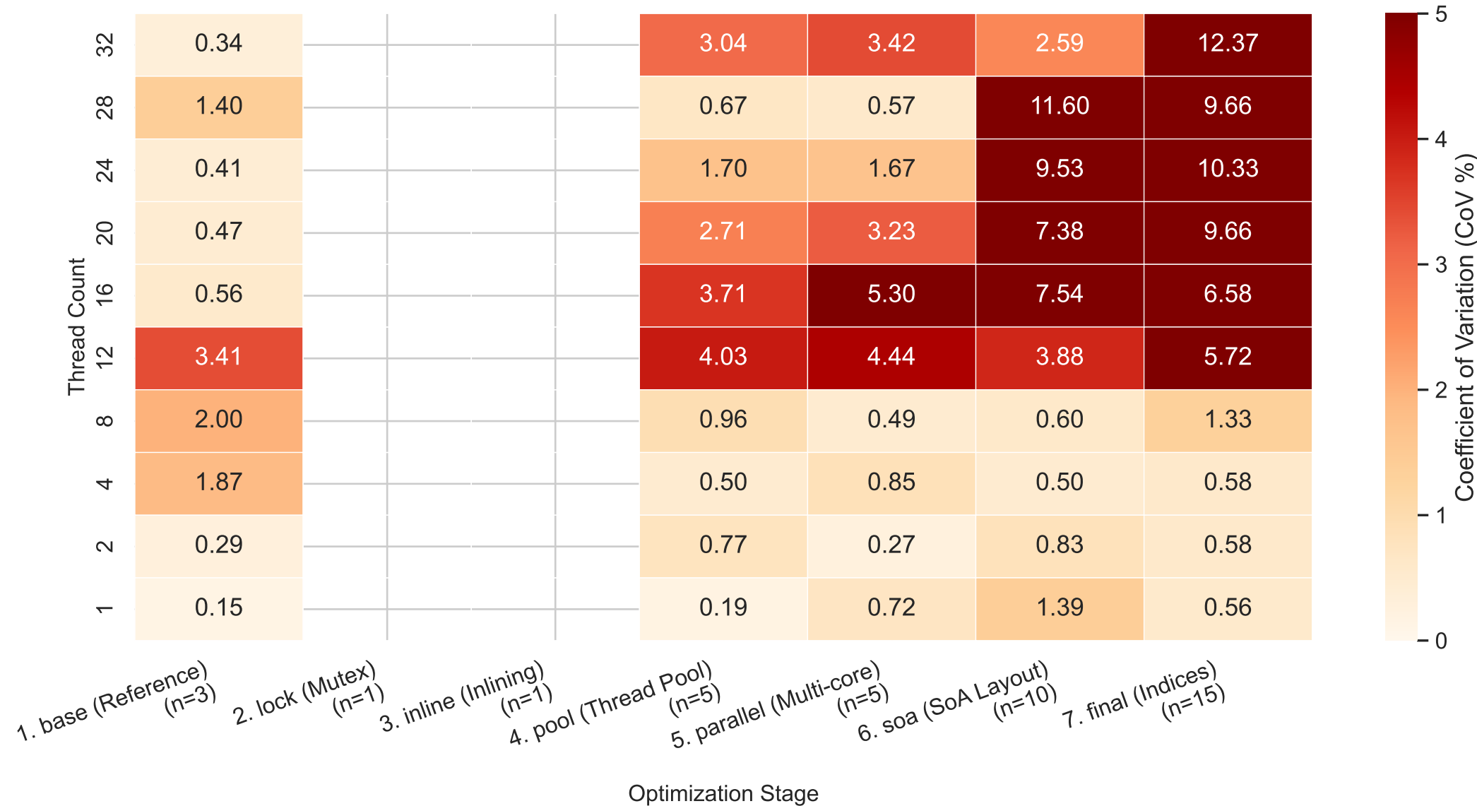
Benchmark Run Stability Heatmap (CoV%) — Scene: 01-Box (CoV Range: 0% - 5%)
