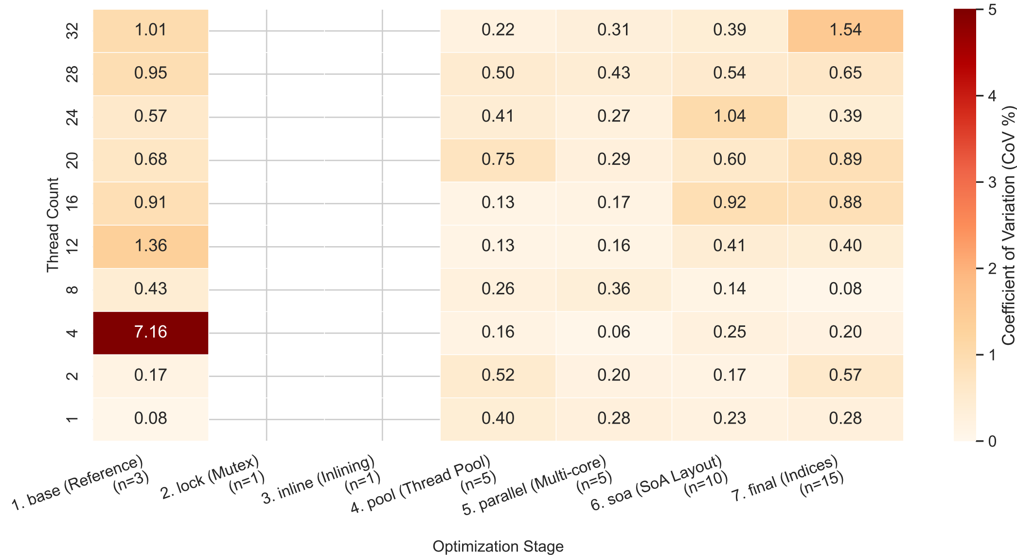
Benchmark Run Stability Heatmap (CoV%) — Scene: 02-Cornell-Box (CoV Range: 0% - 5%)
