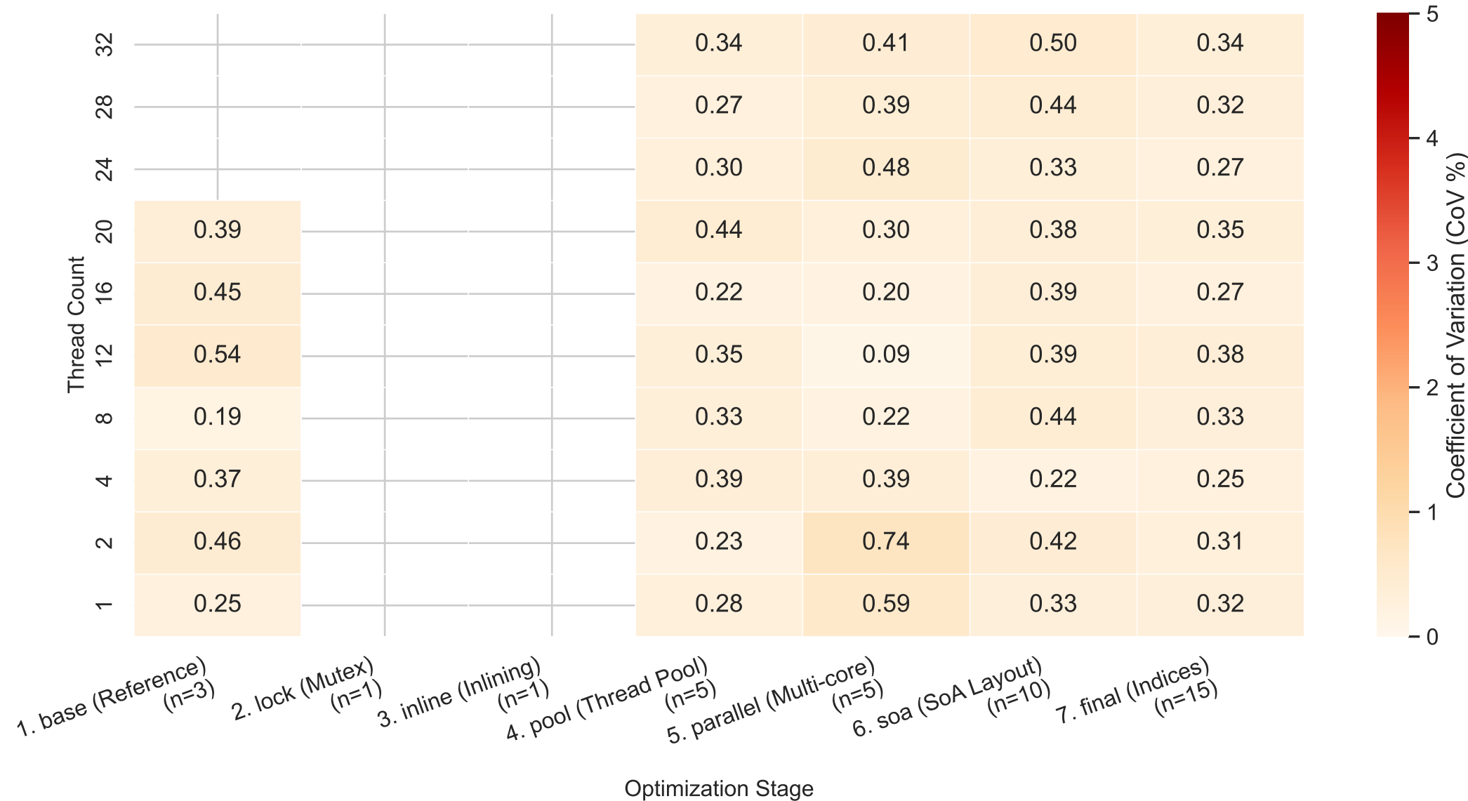
Benchmark Run Stability Heatmap (CoV%) — Scene: 05-Dragon (CoV Range: 0% - 5%)
