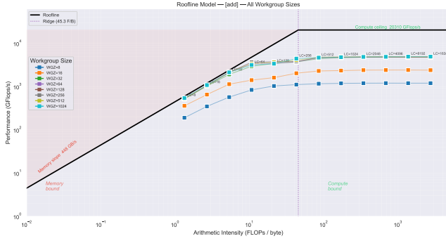
Figure 16: Roofline Model vs Workgroup Size
