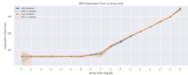
Figure 1: GPU Execution time vs Array Size
