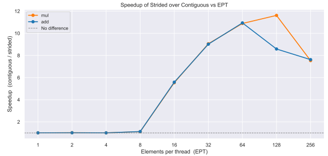
Figure 8: Strided Pattern Speedup vs Contiguous Pattern
