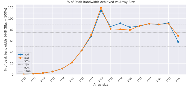
Figure 4: Bandwidth Percentage Utilization vs Array Size
