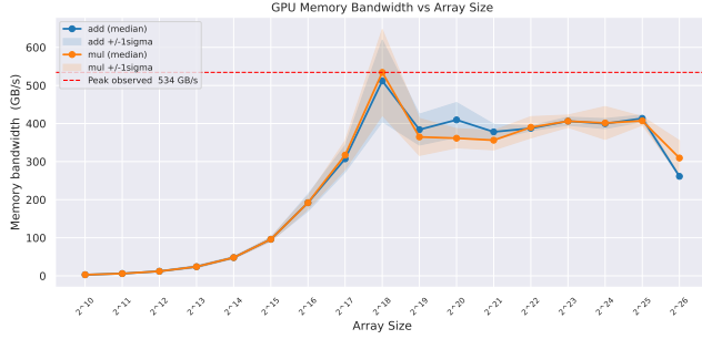
Figure 2: GPU Memory Bandwidth vs Array Size The effective memory bandwidth scales proportionally with array size until reaching a peak at 2^{18} . Beyond this saturation point, throughput begins to decline as the system encounters overheads associated with kernel invocation, kernel inefficiencies and hardware-level memory constraints. At scales of 2^{26} and higher, the results suggest that the GPU enters a memory-bound regime, where performance is strictly limited by the available bus width.
