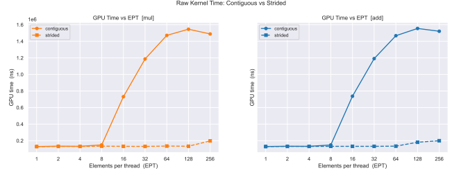
Figure 7: GPU Execution Time vs EPT - mul & add operations - contiguous vs strided pattern
