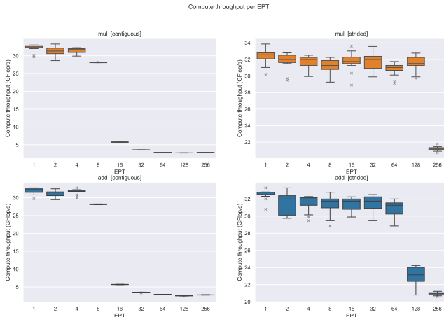
Figure 10: Computational Throughput CI Intervals
