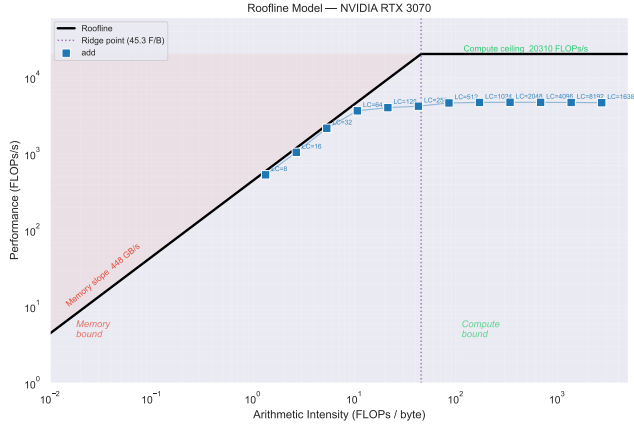
Figure 14: RTX3070 - Roofline Model
