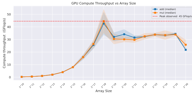
Figure 3: Compute Throughput vs Array Size The trends observed in Figure 3 mirror those in Figure 2. A primary conclusion derived from these figures is that the current kernel implementation is memory-bound, as performance scales in direct correlation with memory bandwidth utilization rather than raw computational capacity.
