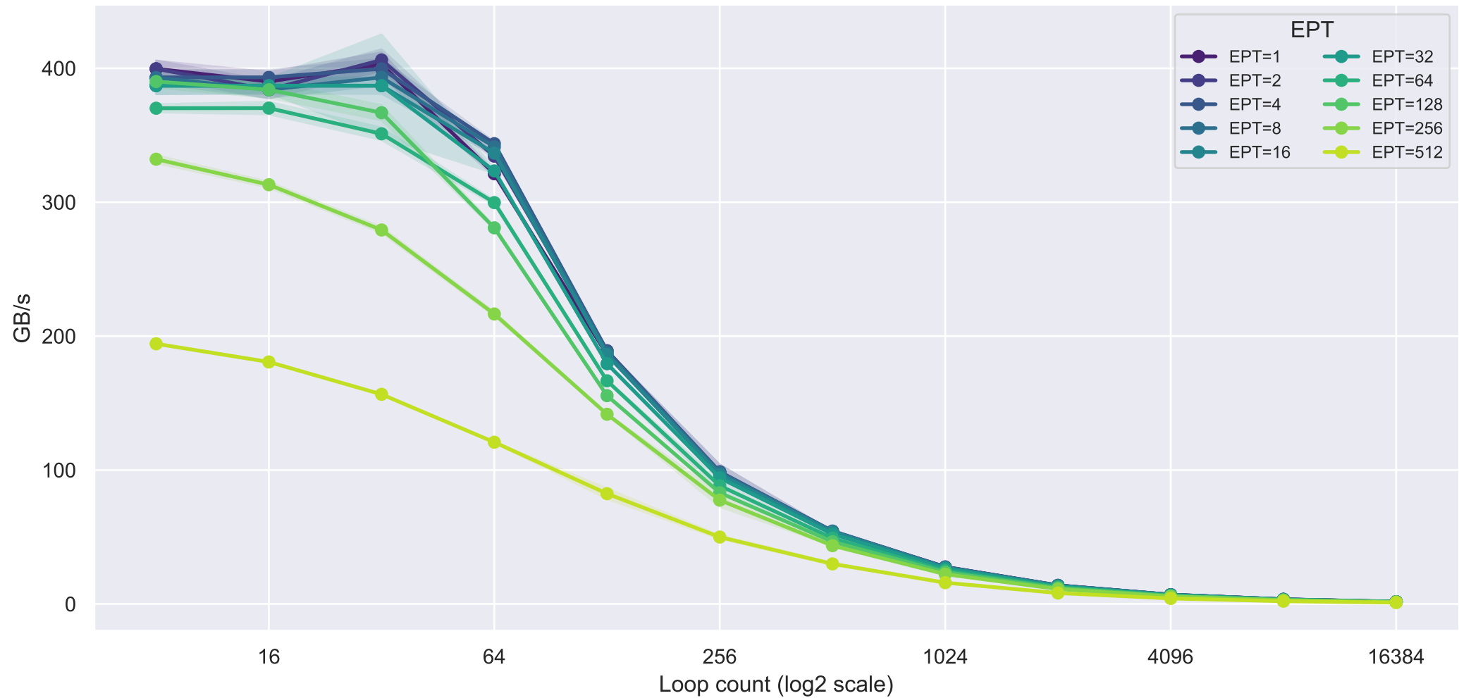
GPU GB/s vs Loop Count — 95% CI, all EPT values [add, strided]
