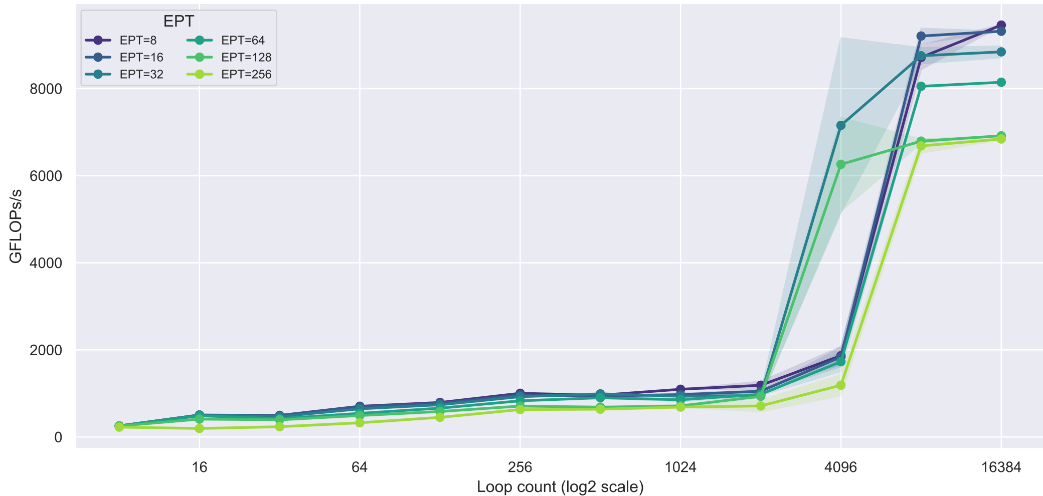
GPU GFLOPs/s vs Loop Count — 95% CI, all EPT values [add, strided]
