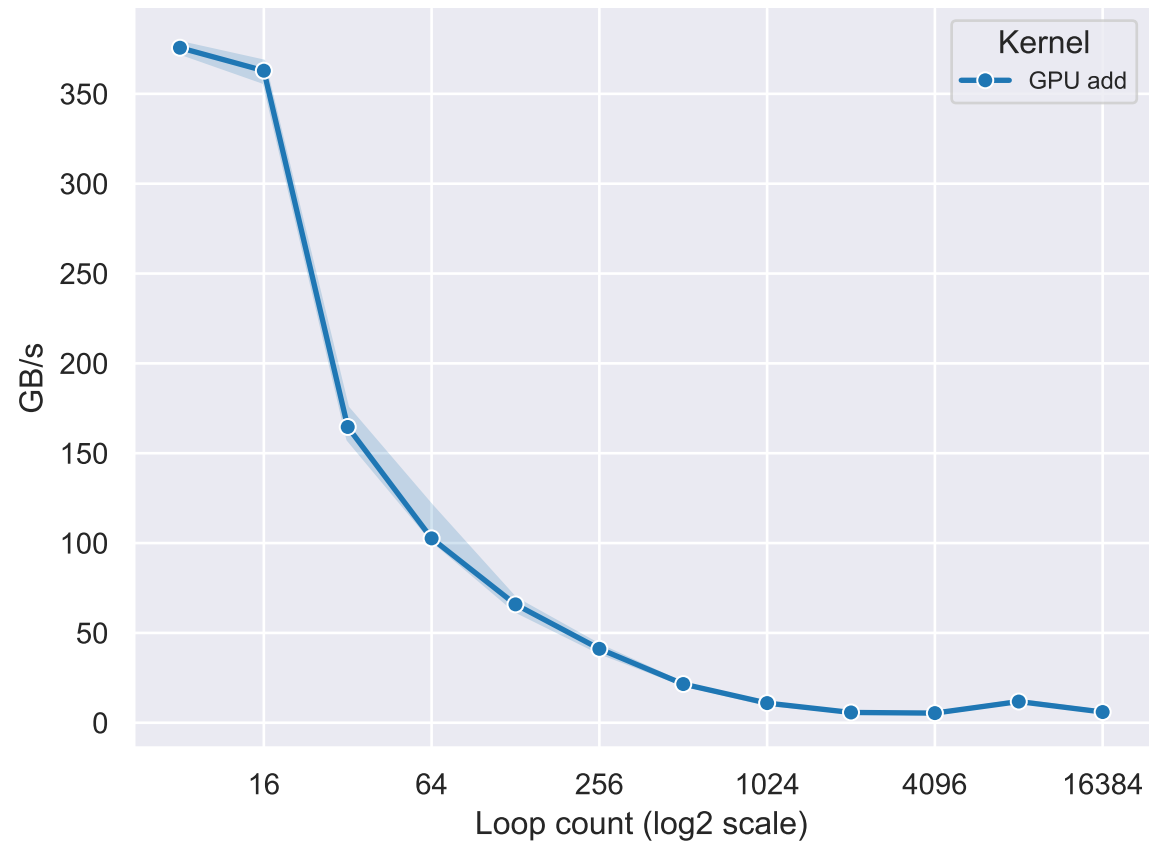
GB/s vs loop count
