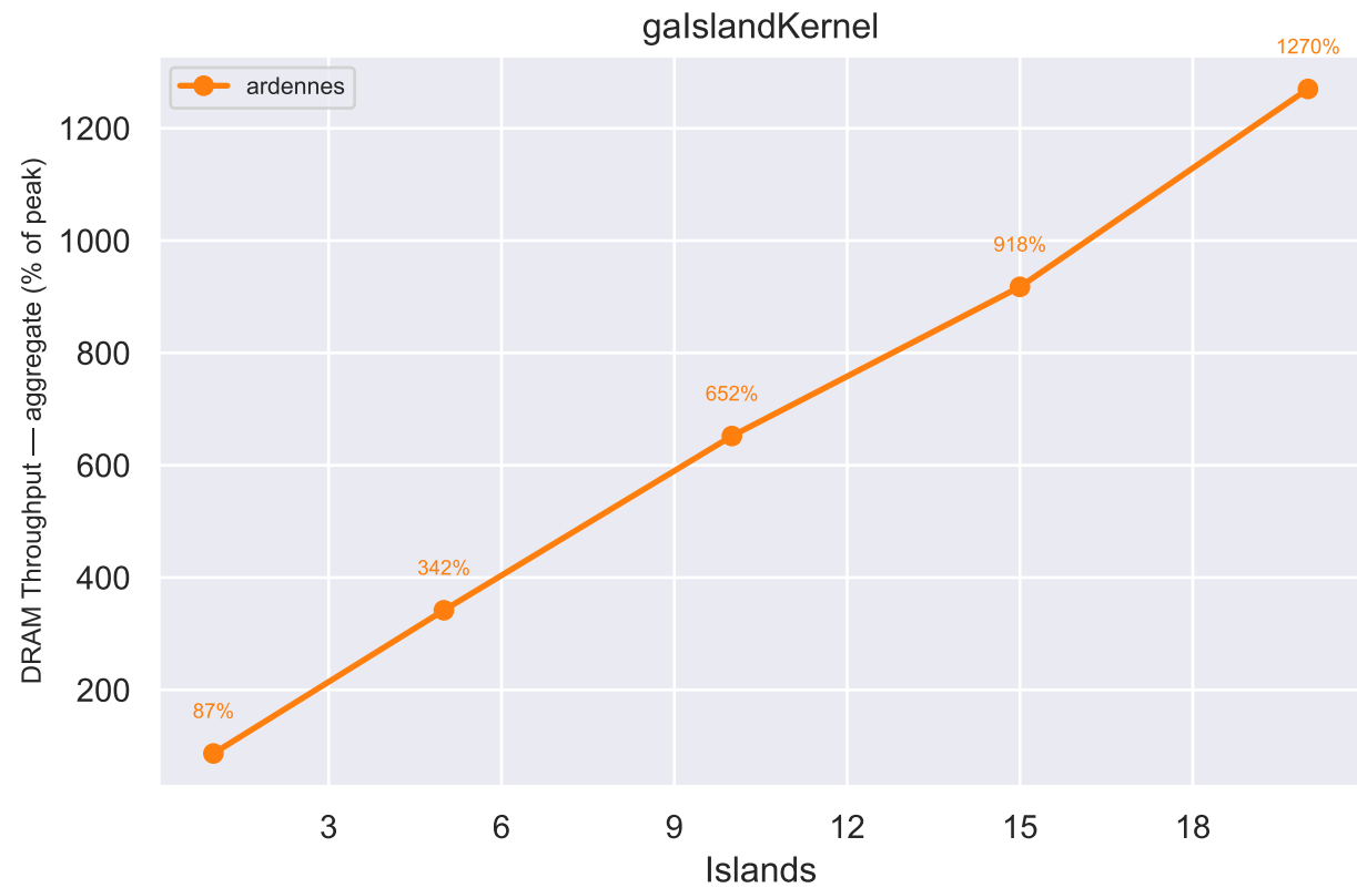
DRAM Throughput Utilization vs. Island Count [ metric is aggregate across all 46 SMs; max theoretical = 4600% ]
