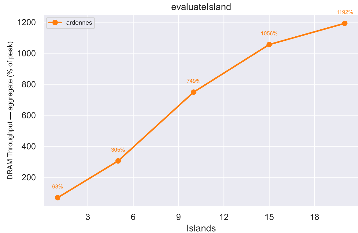
DRAM Throughput Utilization vs. Island Count [ metric is aggregate across all 46 SMs; max theoretical = 4600% ]
