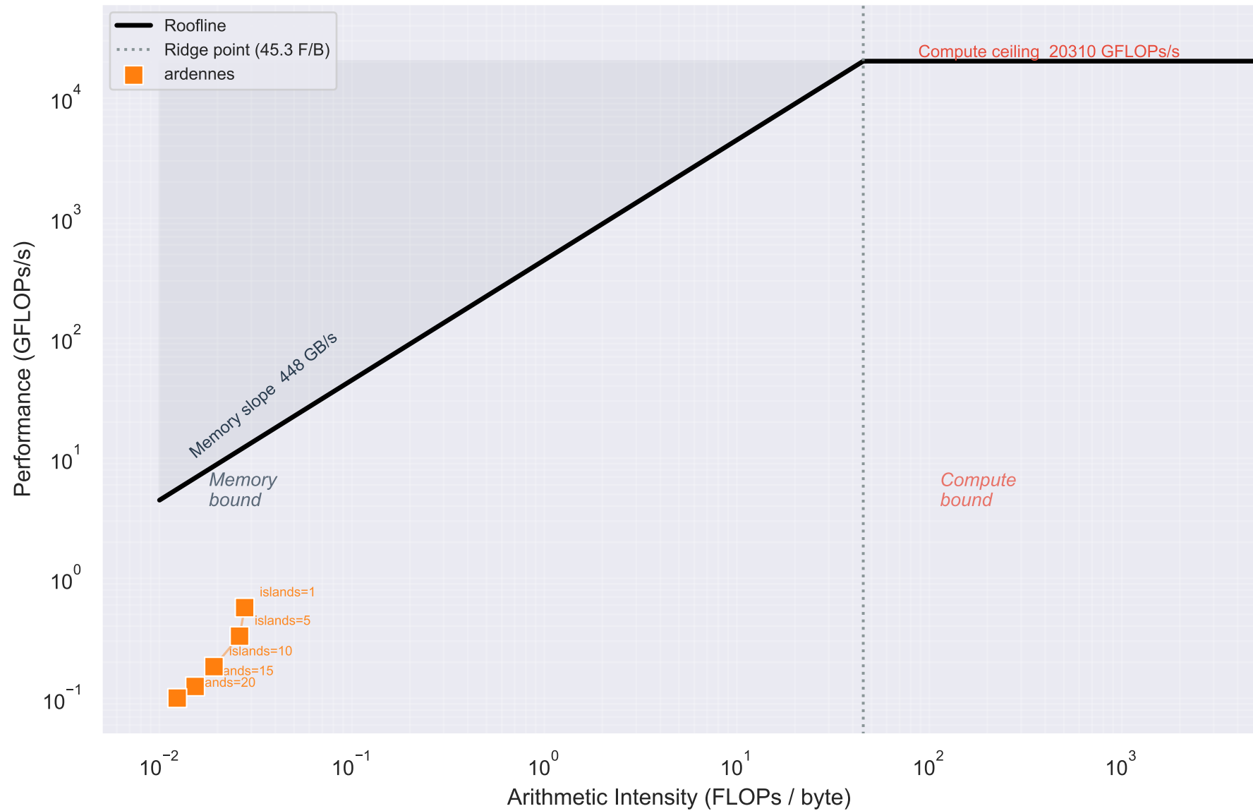
Roofline — FP32 (galslandKernel) — ardennes
