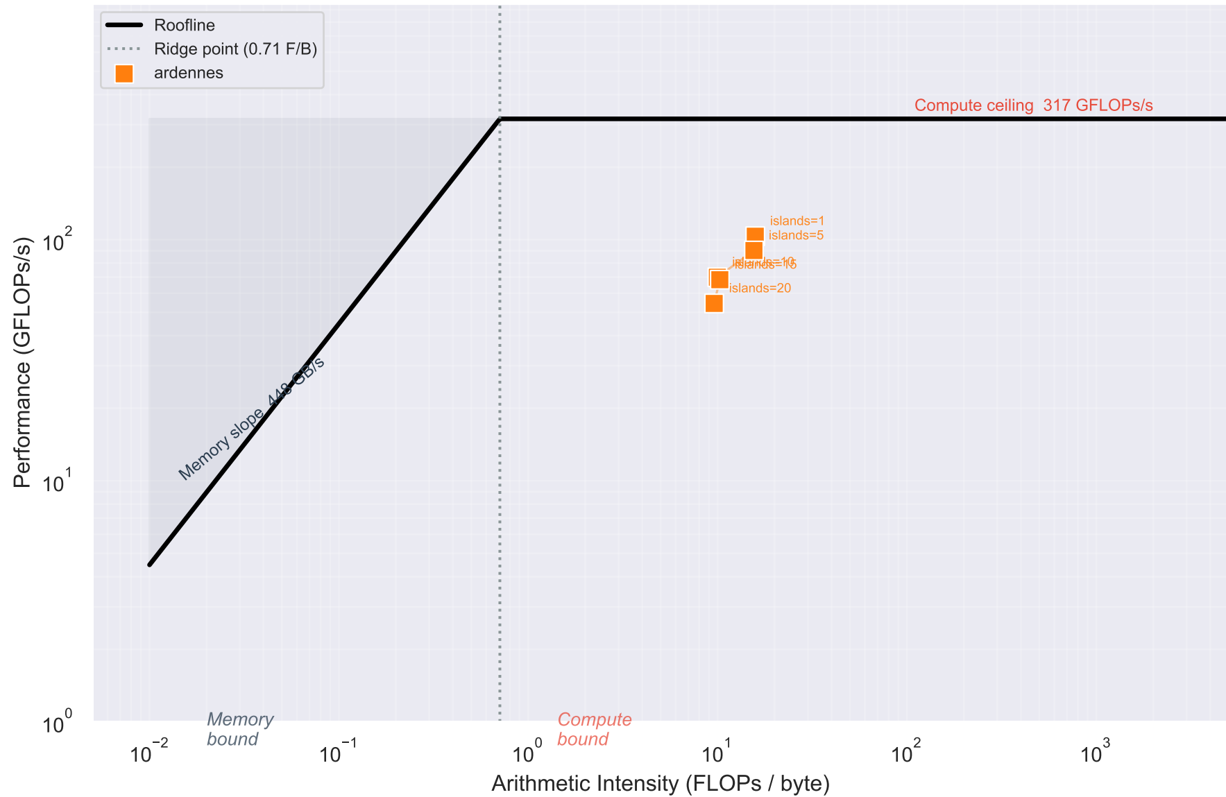
Roofline — FP64 (evaluatelsland) — ardennes
