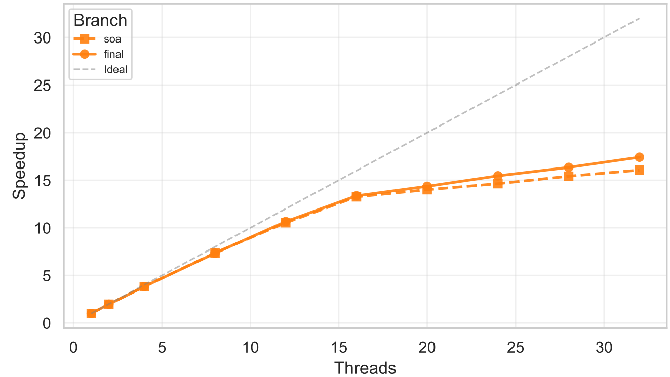
05-Stanford Dragon
