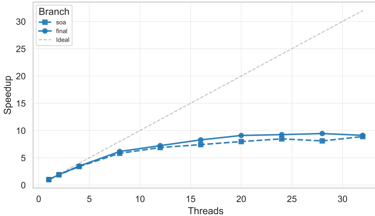
04-Cornell Spheres
