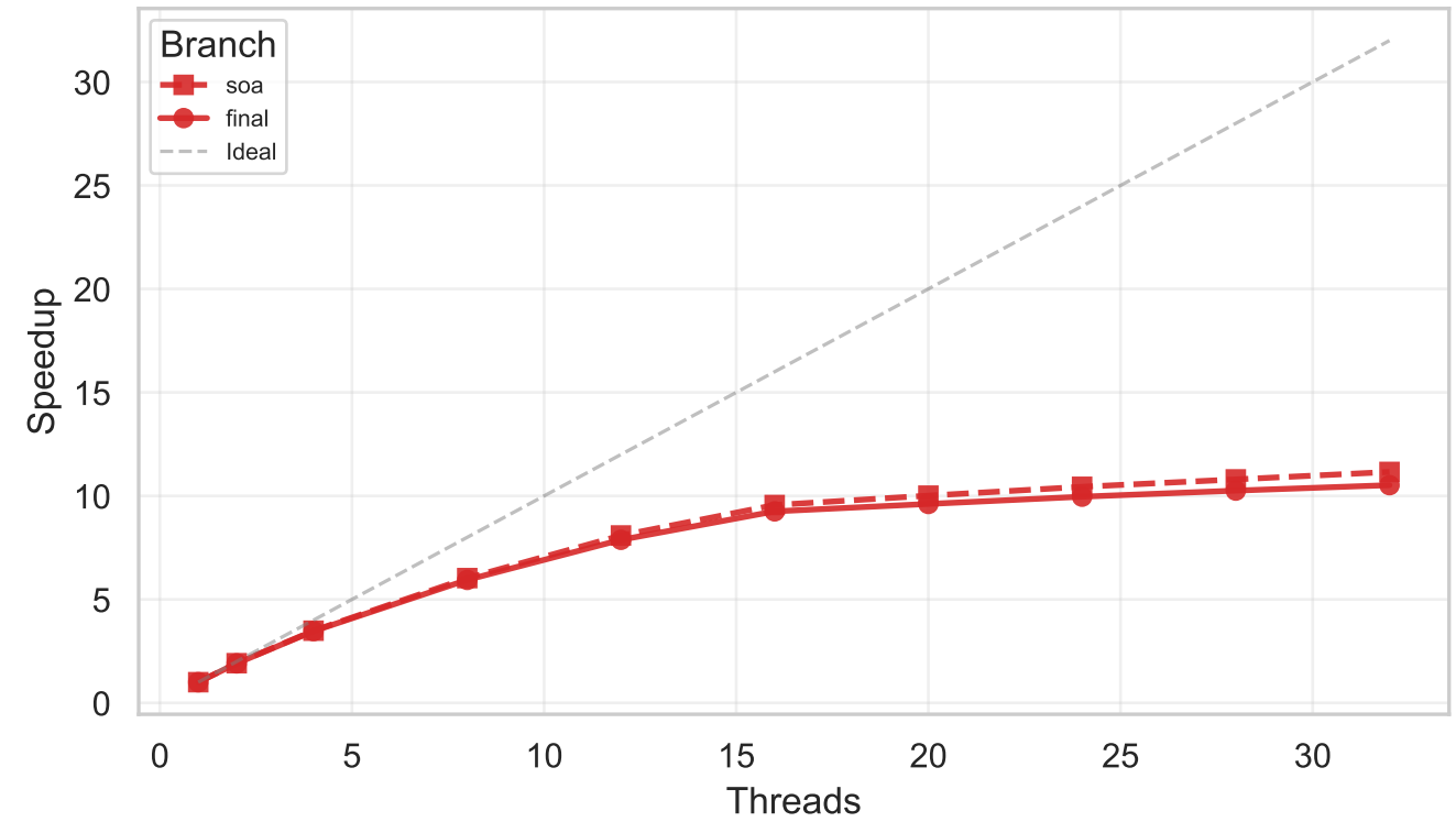
05-Stanford Dragon
