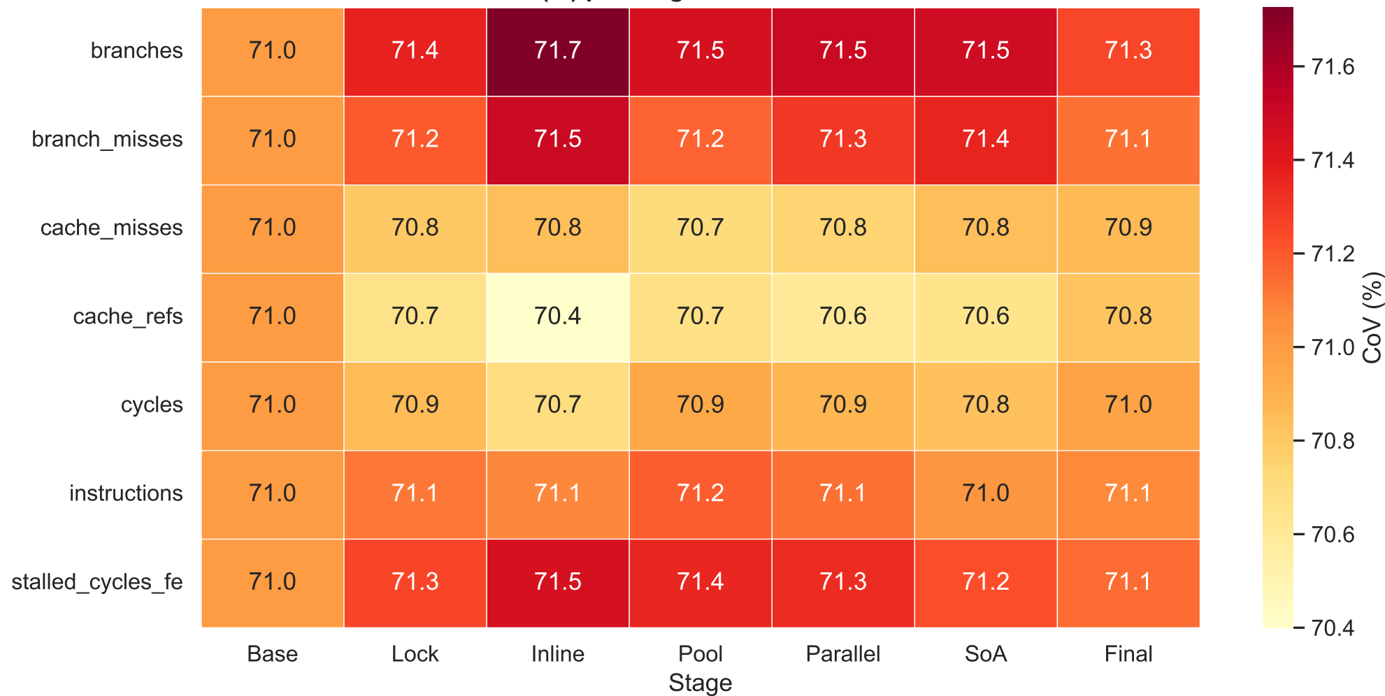
Hardware Counter CoV (%) per Stage — lower = more stable measurement
