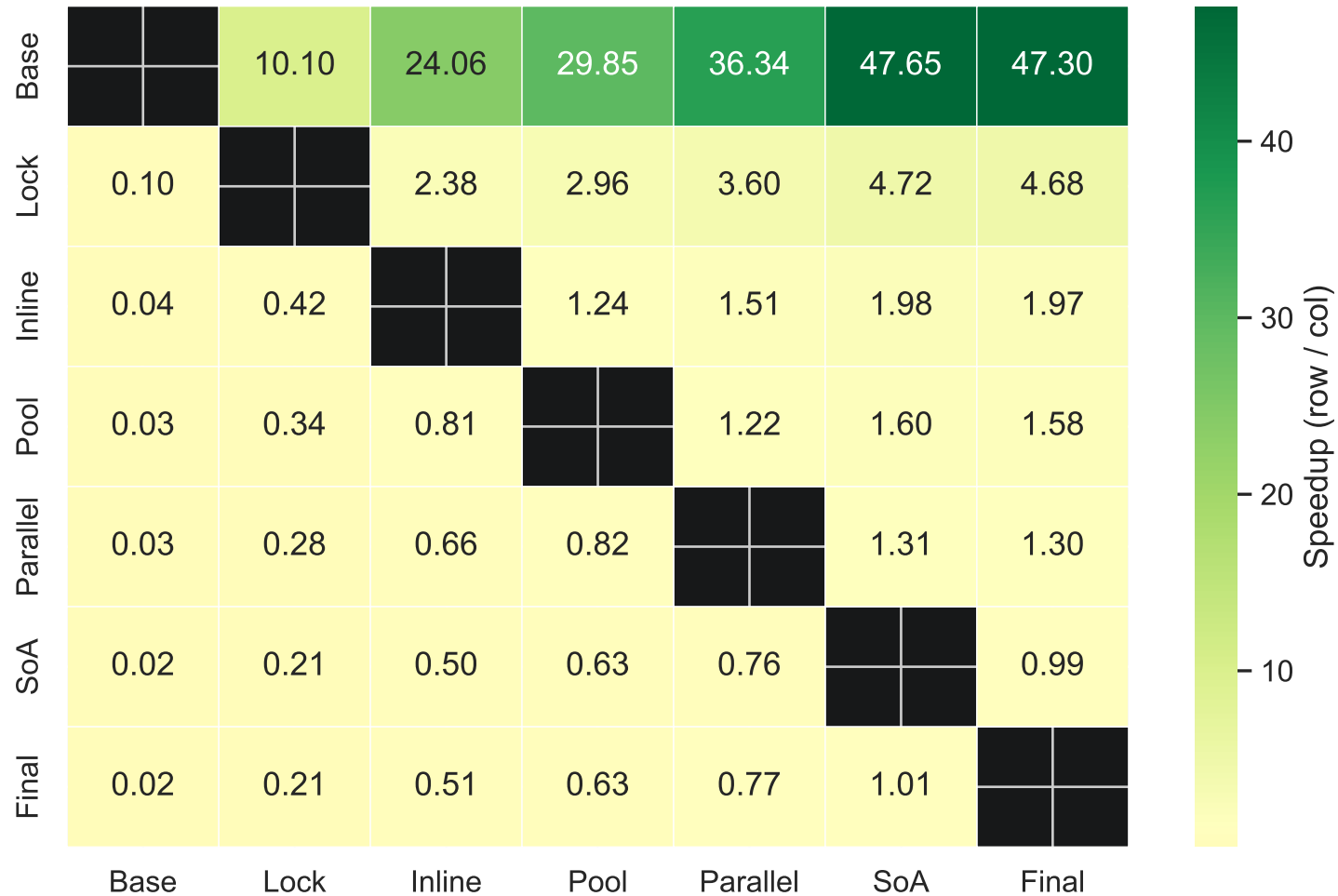
Pairwise Speedup Matrix — 20 thread(s) row faster than col = green (geometric mean over scenes)
