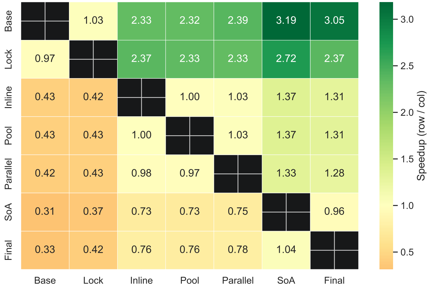
Pairwise Speedup Matrix — 1 thread(s) row faster than col = green (geometric mean over scenes)
