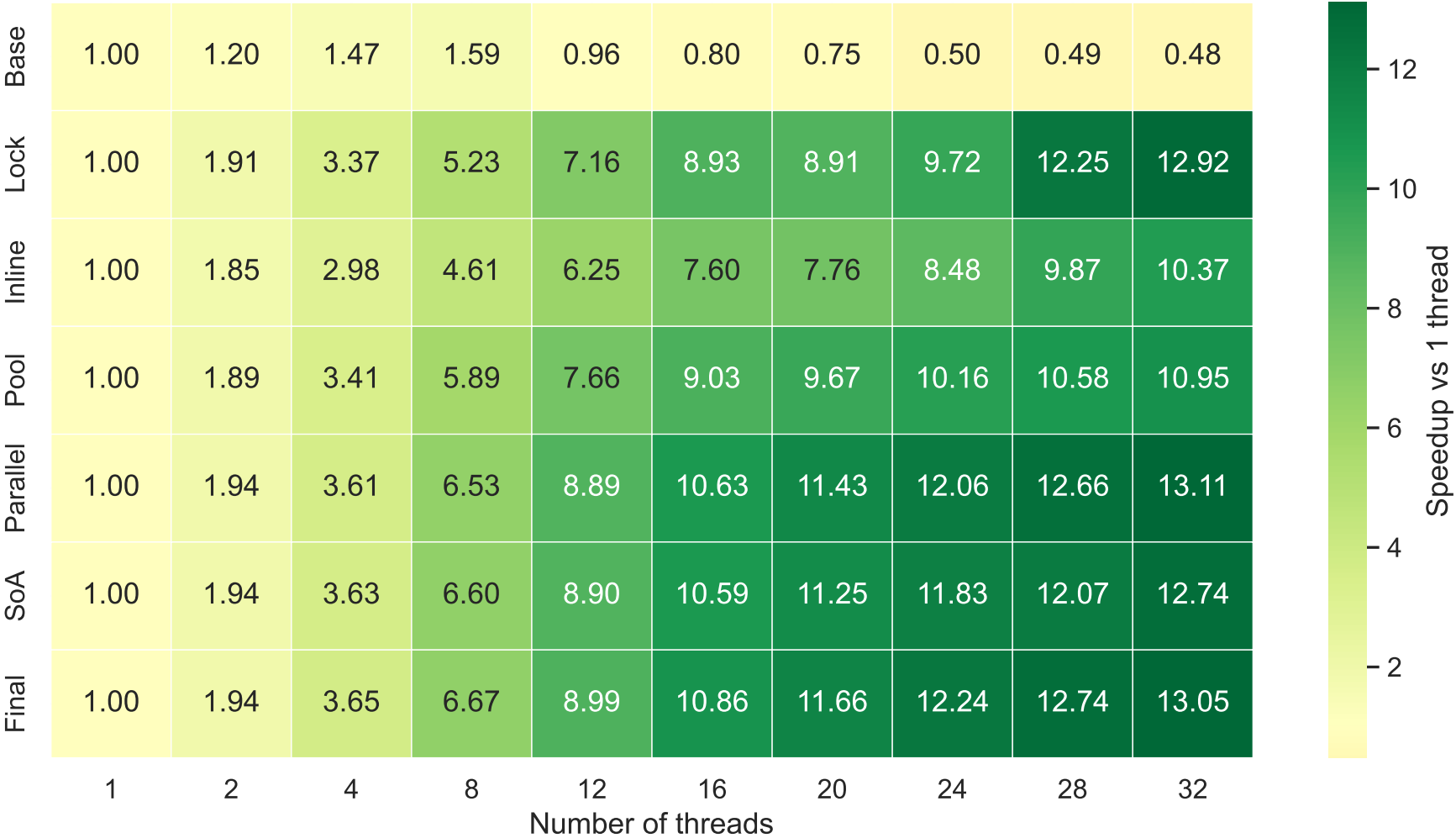
Parallel Speedup per Stage — relative to 1 thread (geometric mean over scenes)
