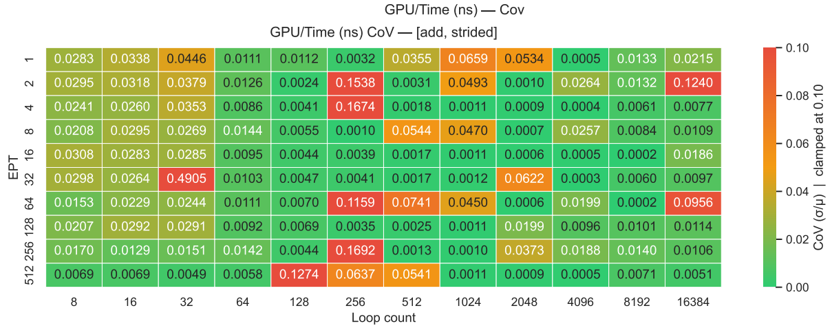
Figure 25: Desktop - Part 3 - GPU Time CoV
