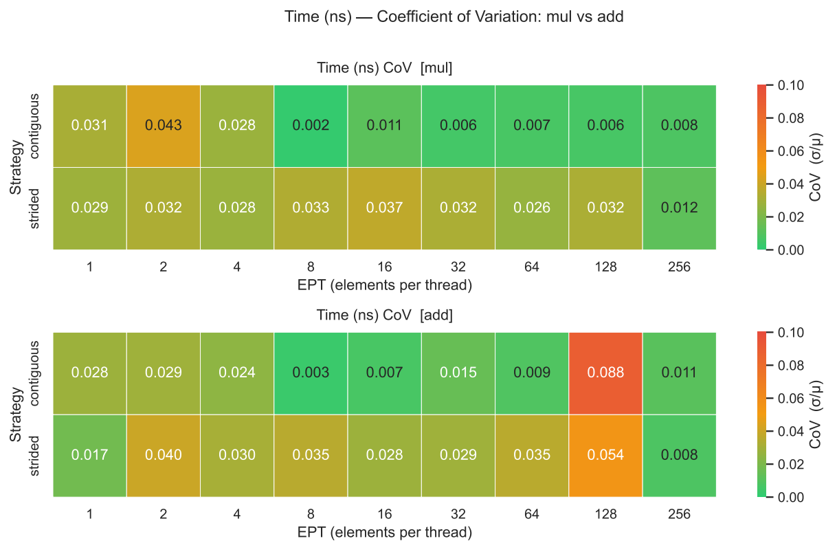
Figure 24: Desktop - Part 2 - GPU Time CoV
