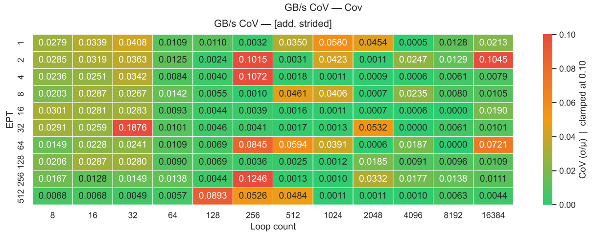
Figure 26: Desktop - Part “” - Memory Bandwidth CoV
