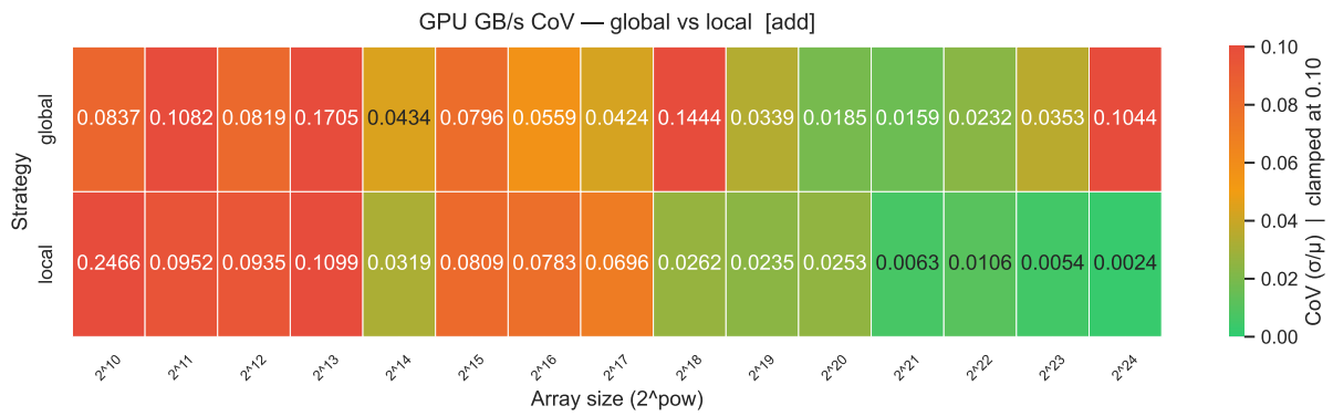
Figure 32: Desktop - Part 4 - Memory Bandwidth CoV
