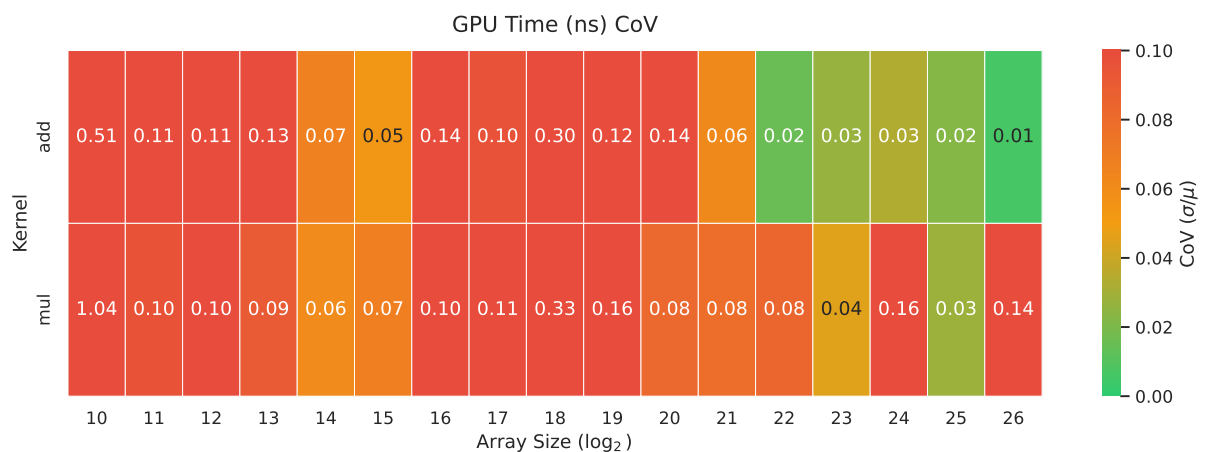
Figure 21: Desktop - Part 1 - GPU Time CoV
