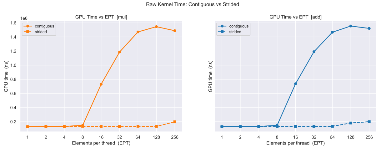
Figure 7: GPU Execution Time vs EPT - mul & add operations - contiguous vs strided pattern Initial observations from the chart suggest that the strided access pattern yields better performance compared to the contiguous pattern. This performance difference is further clarified in Figure 24, where a direct comparison of the two strategies reveals a significant speedup favoring the strided approach as the EPT factor increases.
