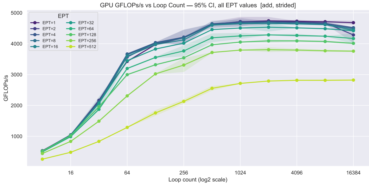
Figure 12: GPU Compute Throughput vs Loop Count
