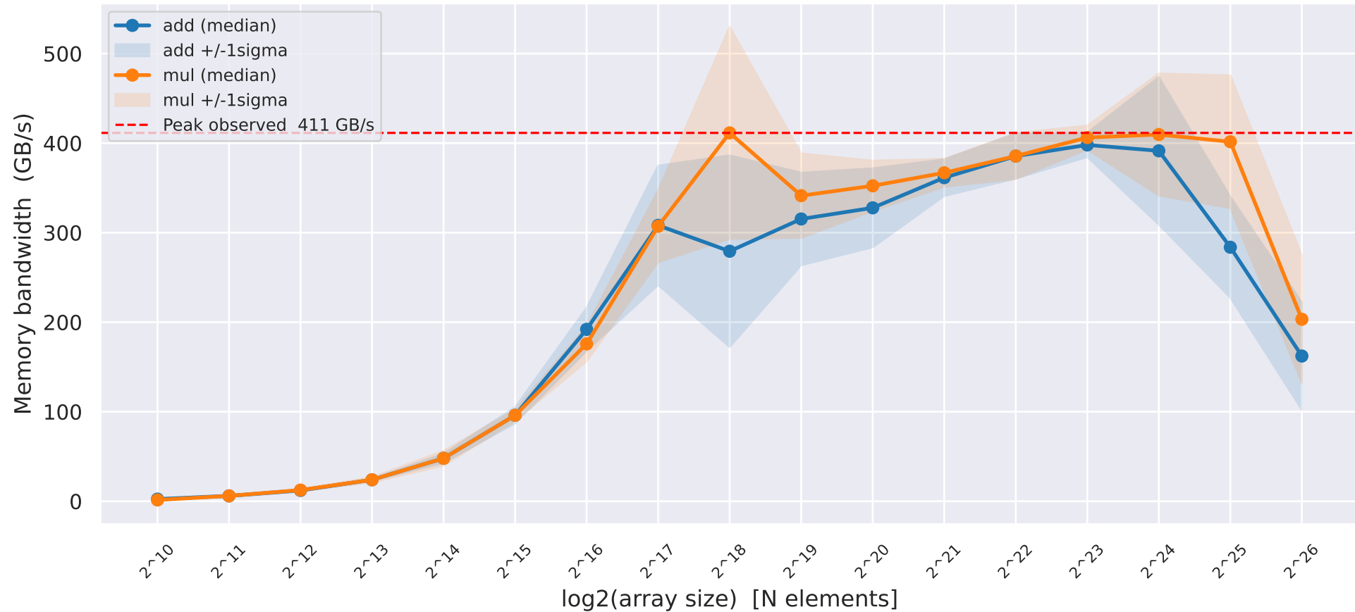
GPU Memory Bandwidth vs Array Size
