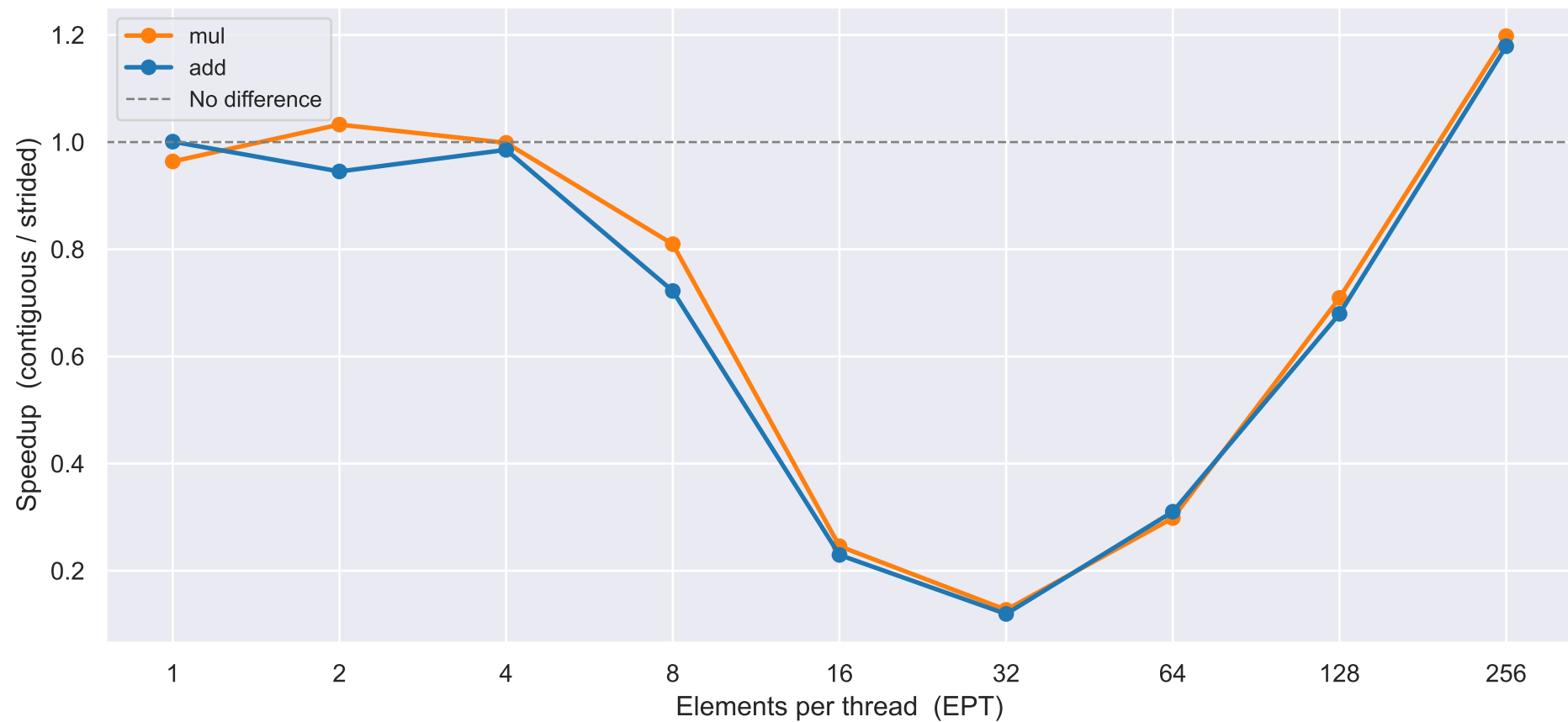
Speedup of Contiguous over Strided vs EPT
