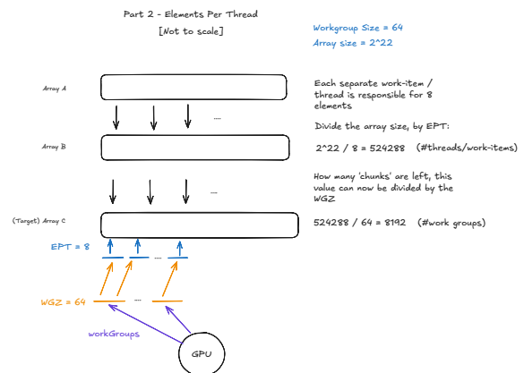
Figure 6: Elements per thread (8) - Work Item Orchestration
