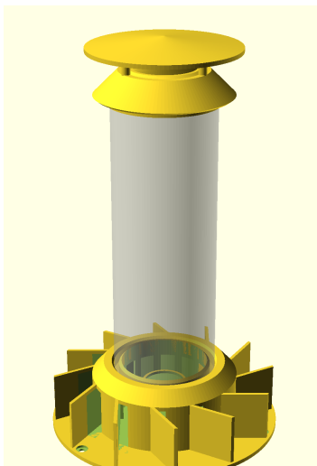
PLATE II — The Wind Tornado: pinwheel intake fins below, stacked-disc venturi cowl above, staked skirt at the foot.
