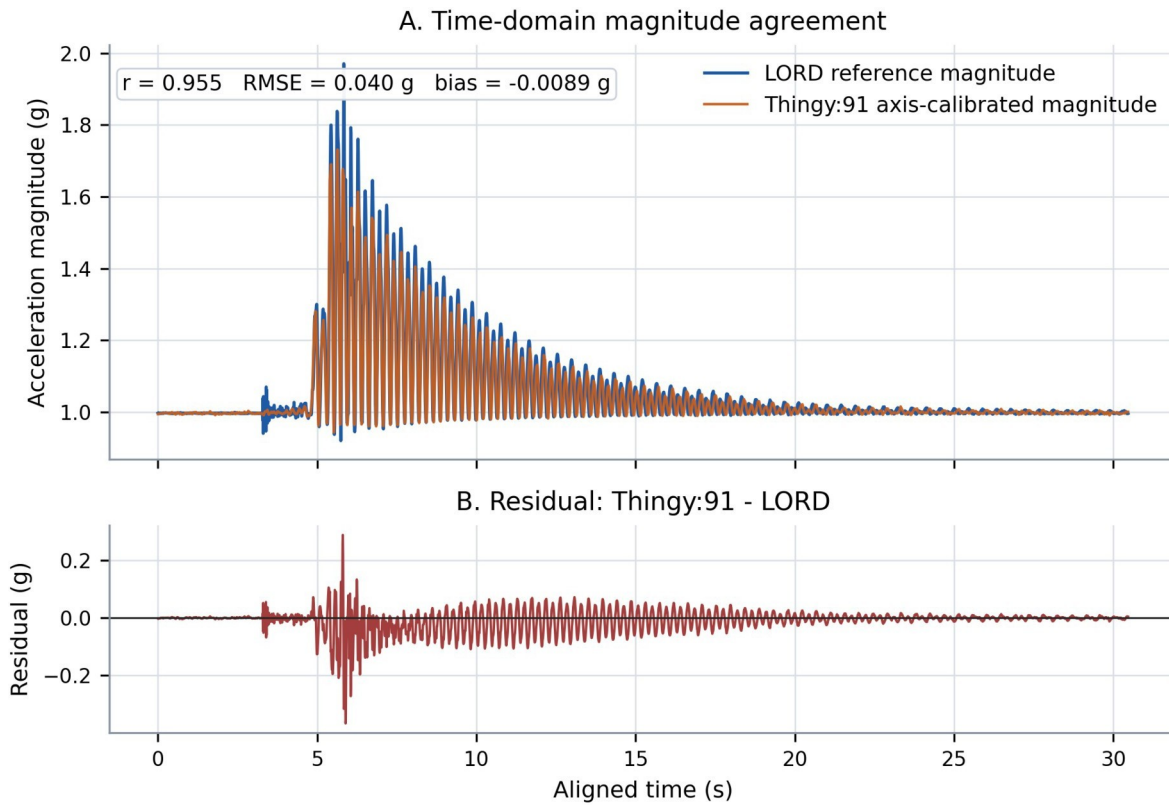
Figure 4.2. Time-domain validation of axis-calibrated magnitude. The upper panel compares LORD reference magnitude with Thingy:91 axis-calibrated magnitude over the aligned validation window; the lower panel shows residual error computed as Thingy:91 minus LORD.
