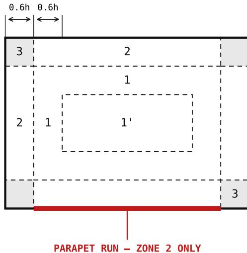
ROOF PLAN – ASCE 7-16 FIG. 30.3-2A
