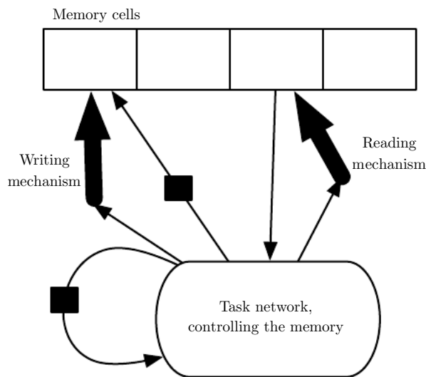
Figure 10.18: A schematic of a network with an explicit memory, capturing some of the key design elements of the neural Turing machine. In this diagram we distinguish the “representation” part of the model (the “task network,” here a recurrent net in the bottom) from the “memory” part of the model (the set of cells), which can store facts. The task network learns to “control” the memory, deciding where to read from and where to write to within the memory (through the reading and writing mechanisms, indicated by bold arrows pointing at the reading and writing addresses).
