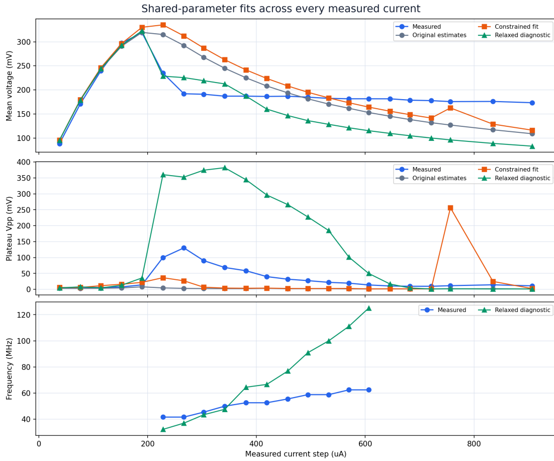
Figure 13: Measured and physics-anchored operating behavior. The complete oscillation window is recovered, while amplitude remains too large and high-current frequency rises too rapidly.
