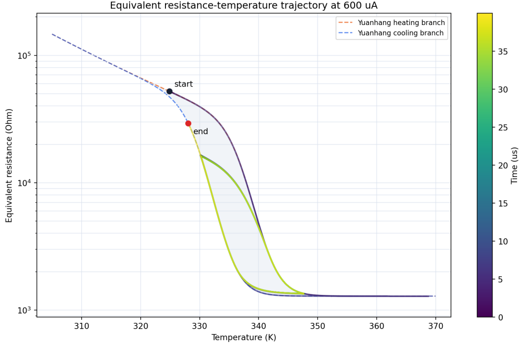
Figure 2: Equivalent resistance versus temperature. The dashed curves and shaded band show Yuanhang’s major heating and cooling hysteresis; color shows progression through the 40 \mu s simulated trajectory.
