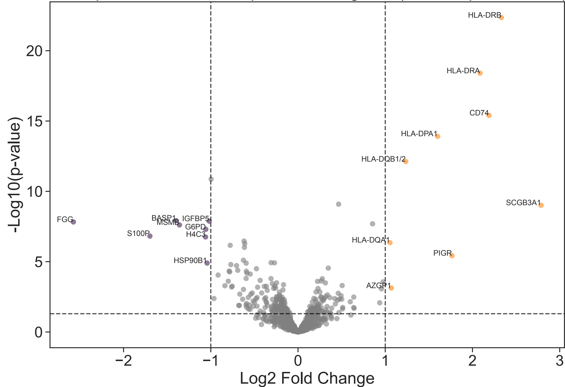
DESeq2 volcano — MHC II positive vs negative (CosMx epithelial cells)
