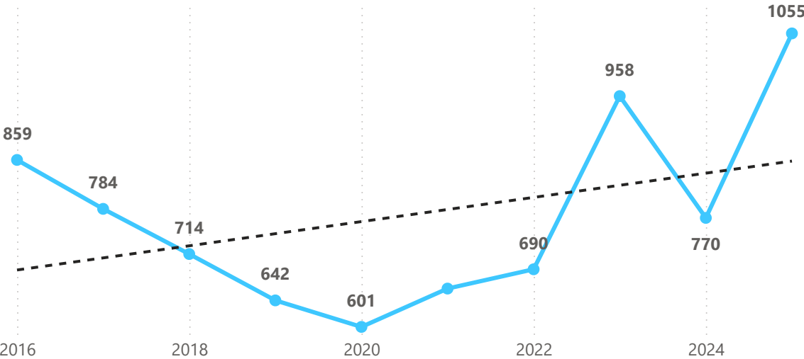
Damage Severity Over Time
