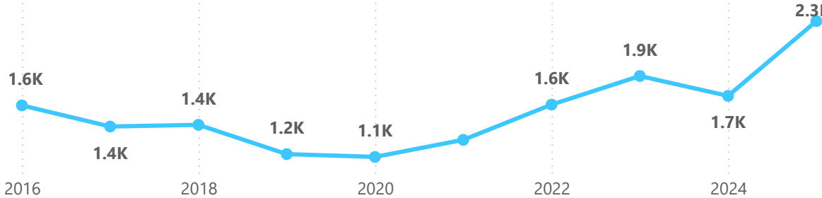
Total Damage Incidents
