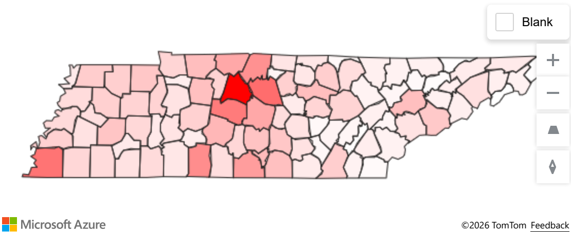
Damage Severity Per County
