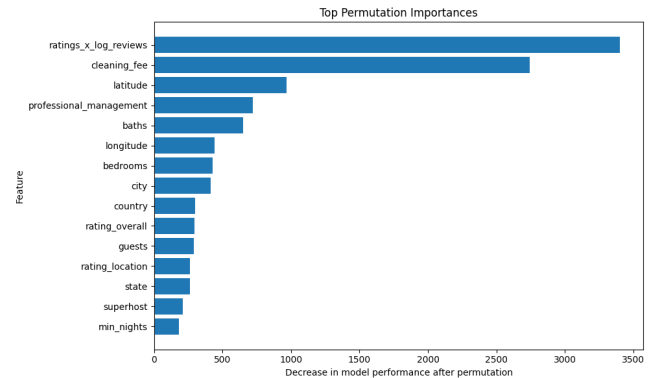
Figure 7: Feature Importance
