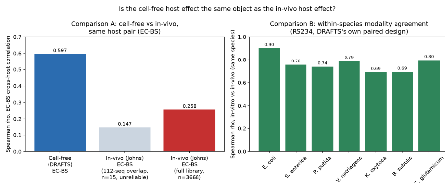
Figure 3 — The DRAFTS modality comparison. Cross-host Spearman \rho , E. coli – B. subtilis pair, cell-free (DRAFTS, N=82 ) vs. in-vivo (this project, full-library reference, N=3,668 ) vs. in-vivo on the small DRAFTS-overlap subset ( N=15 , shown for completeness, not used as evidence — see Section 3.2). No interval shown — each bar is a point Spearman \rho over its full stated N , not a resampled or bootstrapped estimate (DRAFTS provides a single measurement per sequence per species, not a replicate series suitable for bootstrapping the correlation itself beyond what N already reflects). Full data: out/results/gate10_modality_comparison.json . Script: scripts/91_drafts_modality_comparison.py .
