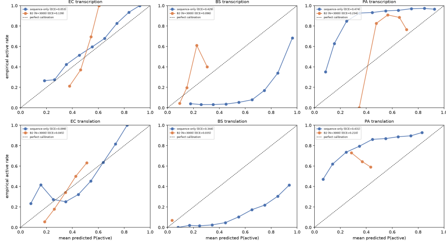
Figure 6 — Off-distribution calibration collapse. Reliability diagrams for the zero-shot active/inactive classifier, all three primary hosts and both readouts, with Expected Calibration Error per panel.
