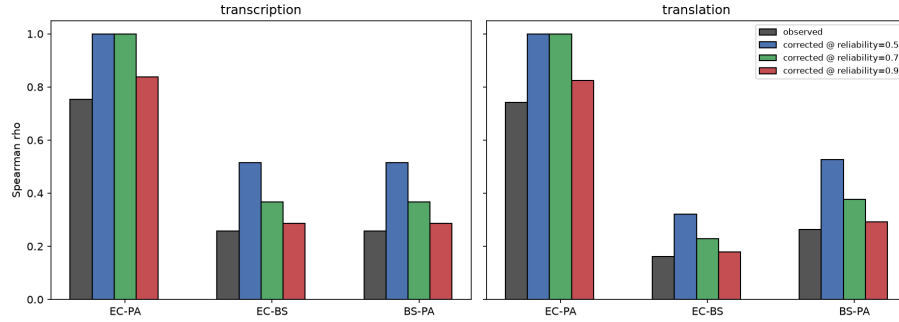
Figure 1: Figure 1 — Raw cross-host measurement correlation, with disattenuation correction. Spearman \rho for all three pairs, both readouts, co-active regime, raw and disattenuation-corrected. Co-active N per pair: transcription EC-BS 3,668, EC-PA 9,741, BS-PA 2,099; translation 866, 3,826, 314. No resampled interval — these are population correlations, and the correction is a deterministic formula shown at three reliability levels (0.5/0.7/0.9) as a sensitivity grid.
