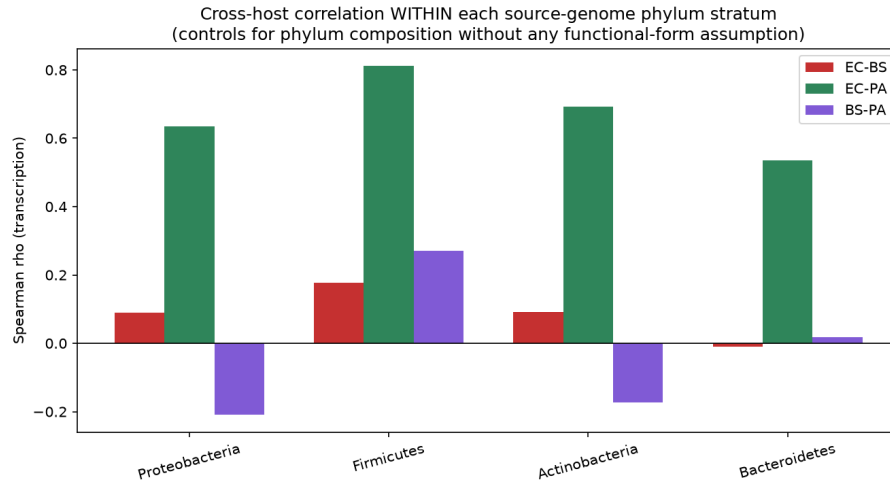
Figure 3: Figure 2b — Phylum stratification. The same contrast computed within Proteobacteria and within Firmicutes separately, as an assumption-free check on the GC control.
