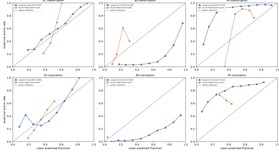
Figure 7: Figure 6 — Off-distribution calibration collapse. Reliability diagrams for the zero-shot active/inactive classifier, all three primary hosts and both readouts, with Expected Calibration Error per panel.
