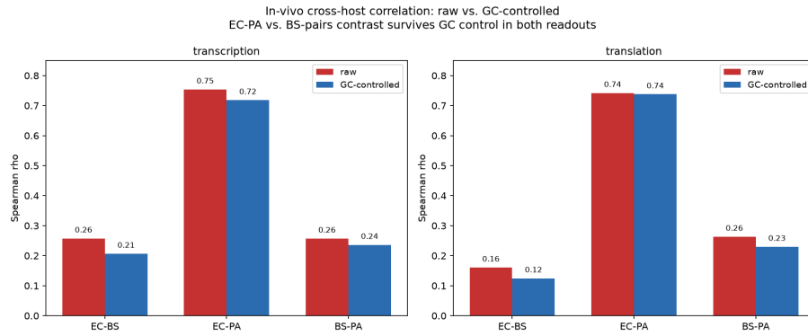
Figure 2: Figure 2a — GC-composition control. Raw vs. GC-controlled Spearman \rho , all three pairs and both readouts, partial-correlation control confirmed independently by closed-form formula and rank-residual regression.
