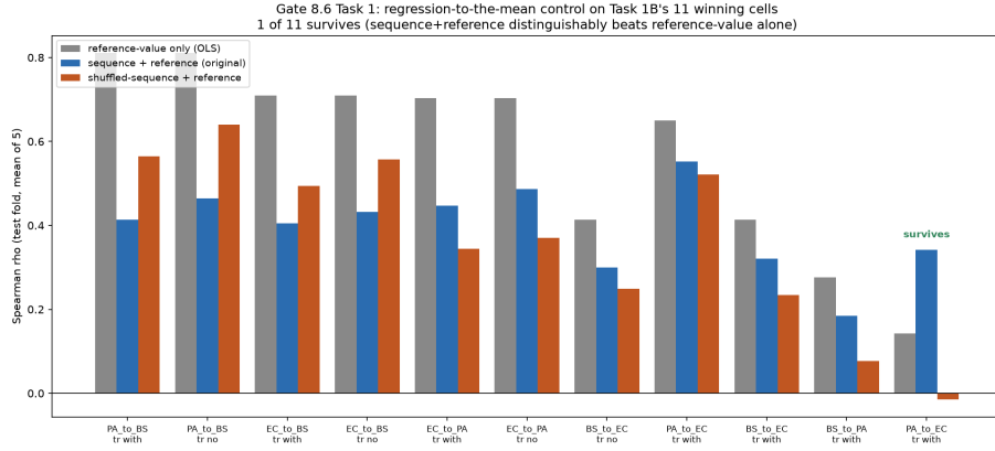
Figure 9: Figure 8 — The shift-prediction retraction. Original model vs. reference-value-only baseline vs. shuffled-sequence control, Spearman \rho against true shift, for the originally-reported winning cells. N ranges 294–9,609 per cell (for example, EC→BS transcription 3,589; EC→PA 9,609; BS→PA translation 294). Single point estimates on the held-out fold; the retraction rests on the comparisons, not on interval non-overlap.
