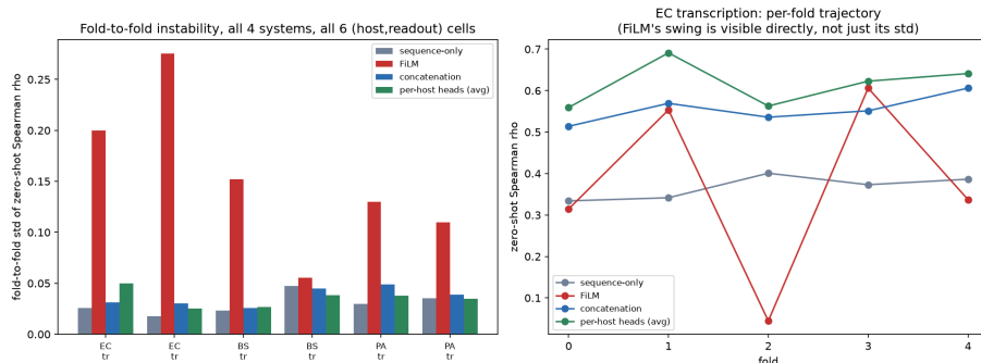
Figure 8: Figure 7 — FiLM fold-to-fold instability. Fold-to-fold standard deviation of zero-shot \rho across all 6 (host, readout) cells and all four systems. No interval: this figure reports variance itself, computed across N = 5 folds per cell.
