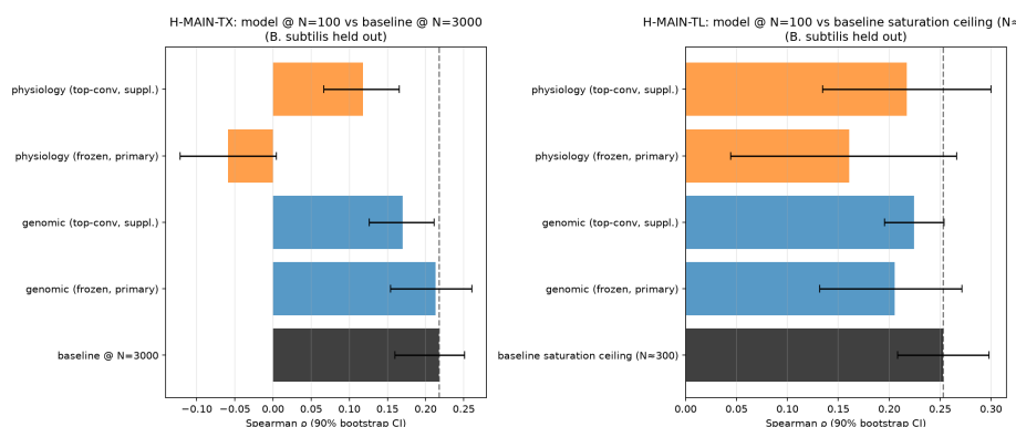
Figure 5: Figure 4 — The pre-registered kill gate (H-MAIN). Model vs. per-host baseline across all 8 primary comparisons, with 90% percentile bootstrap intervals (10,000 resamples, hierarchical over folds then draws). None met the pre-registered bar.
