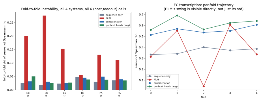
Figure 7 — FiLM fold-to-fold instability. Fold-to-fold standard deviation of zero-shot \rho across all 6 (host, readout) cells and all four systems. No interval: this figure reports variance itself, computed across N = 5 folds per cell.
