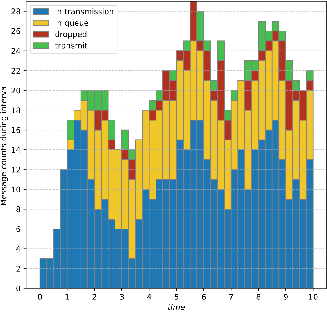
Duration=10, Clients count=1, Client's \lambda =12, Servers count=1, Q=8
