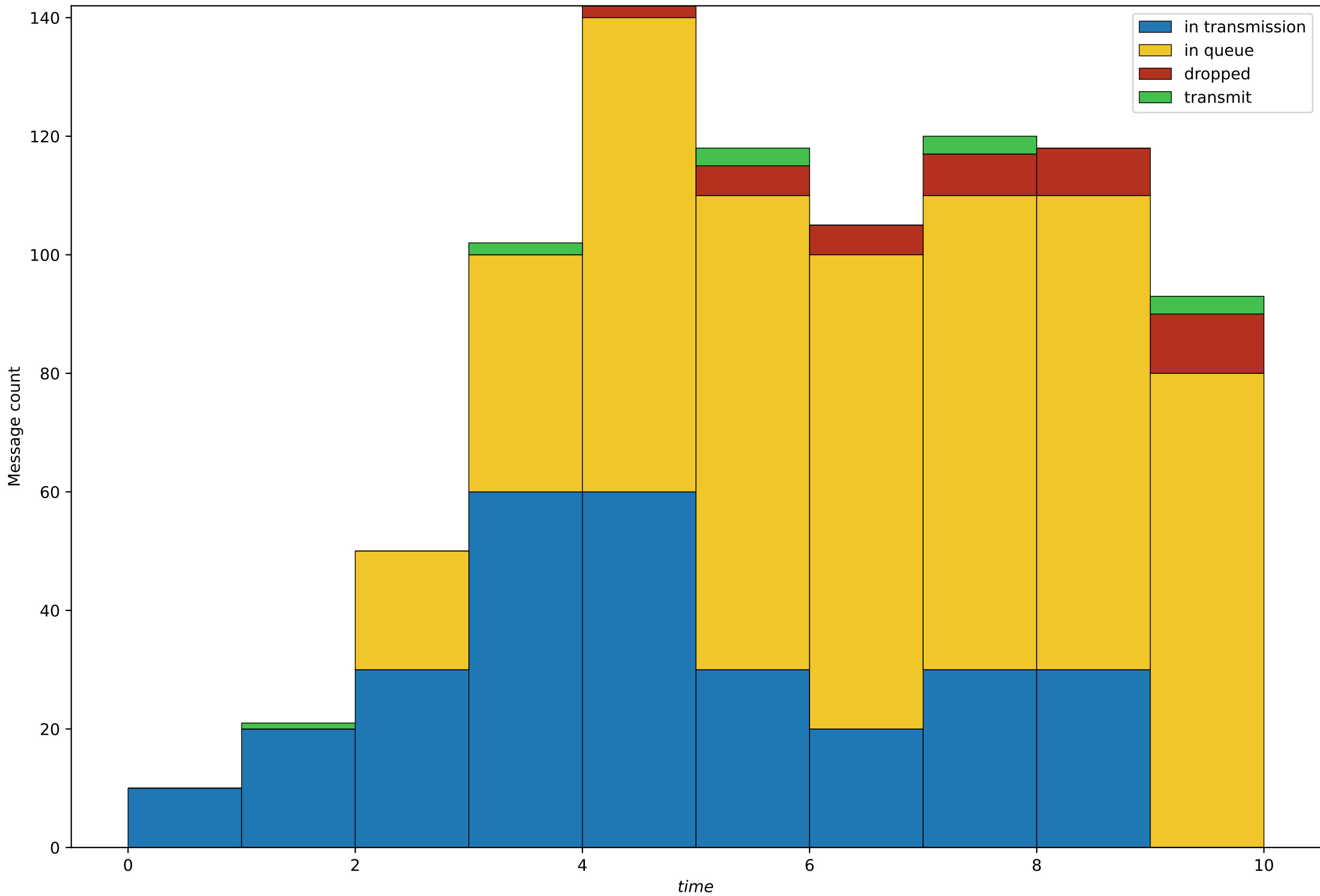
Duration=10, Clients count=1, Client's \lambda=4 , Servers count=1, Q=8
