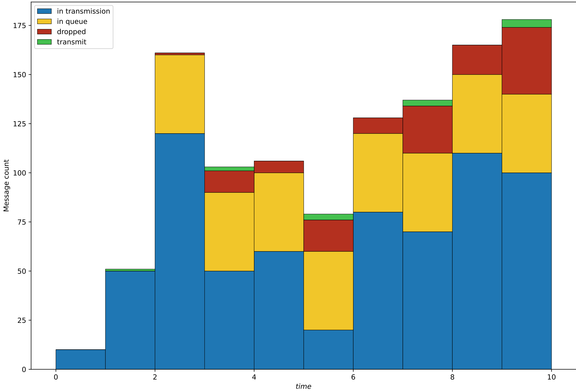
Duration=10, Clients count=1, Client's \lambda=8 , Servers count=1, Q=4
