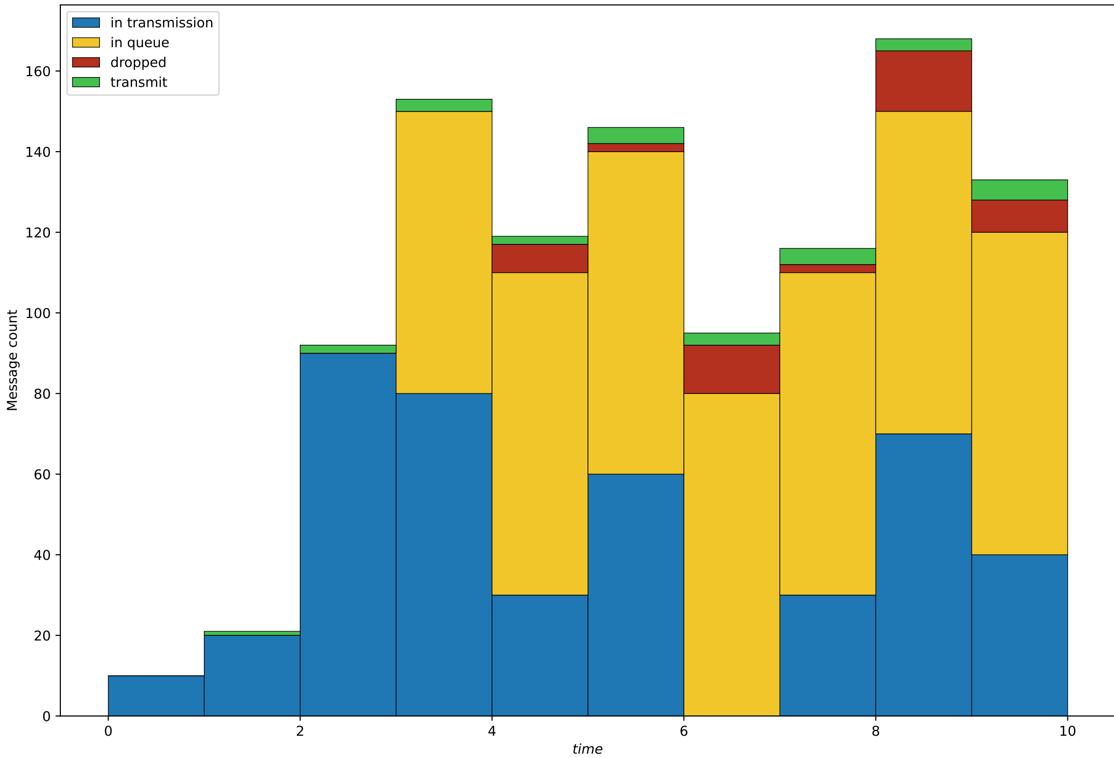
Duration=10, Clients count=1, Client's \lambda=6 , Servers count=3, Q=8
