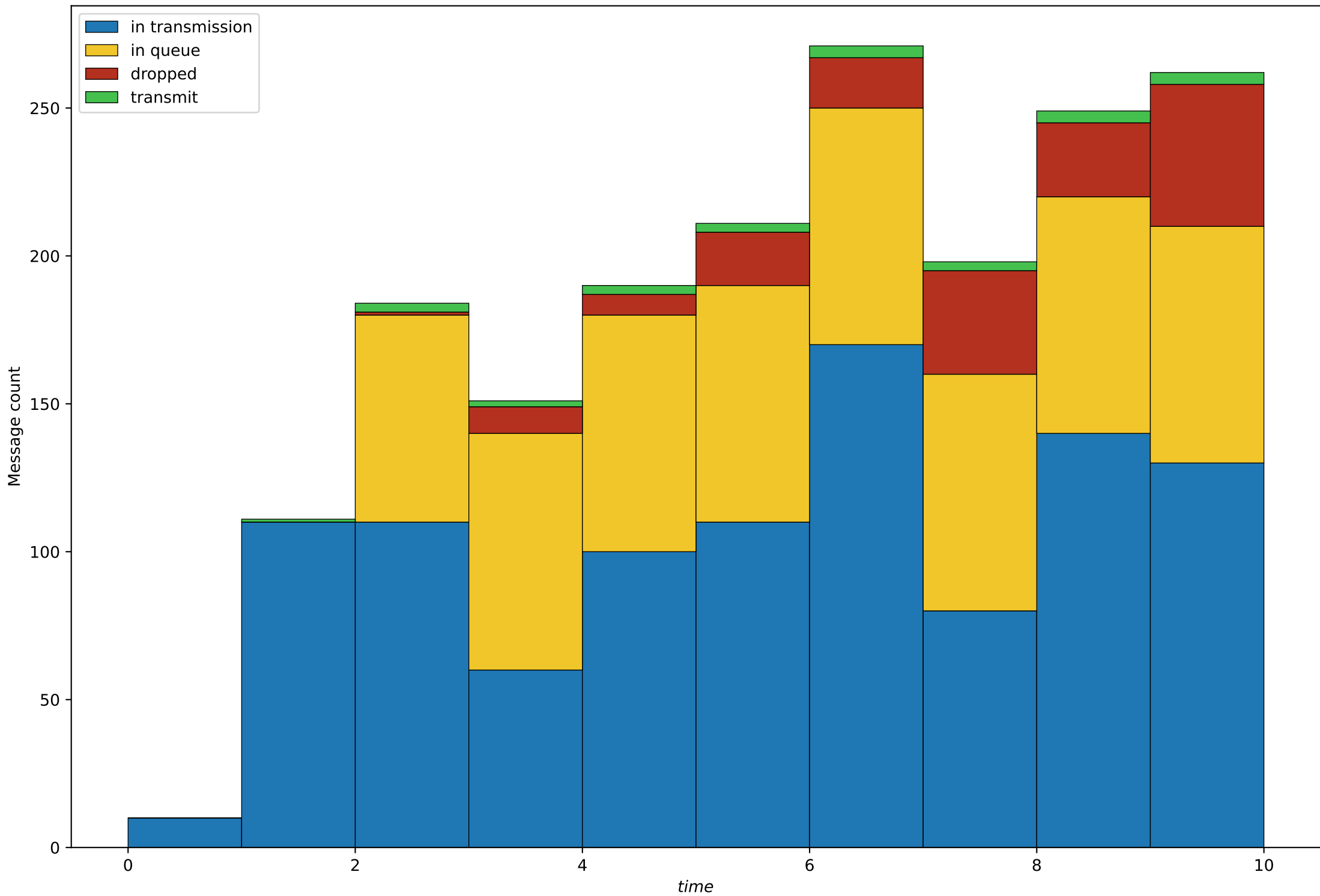
Duration=10, Clients count=1, Client's \lambda=12 , Servers count=3, Q=8
