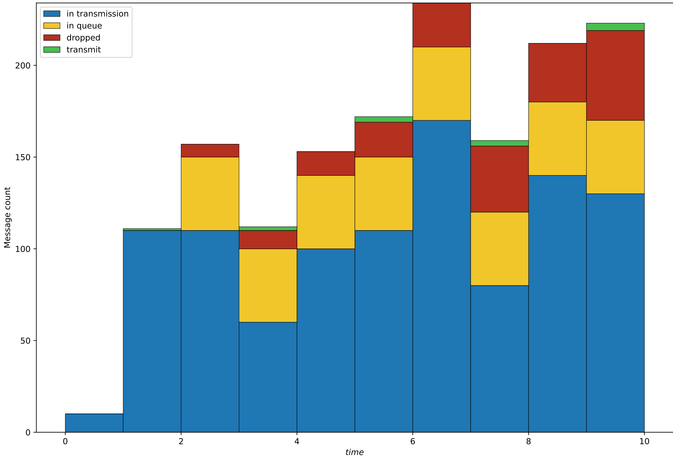
Duration=10, Clients count=1, Client's \lambda=12 , Servers count=1, Q=4
