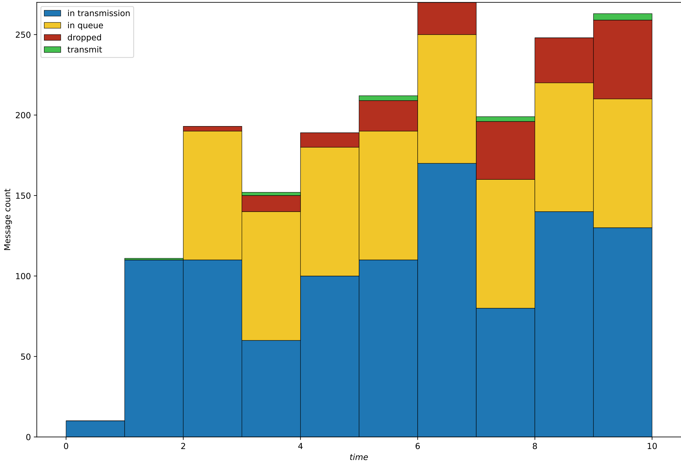
Duration=10, Clients count=1, Client's \lambda=12 , Servers count=1, Q=8
