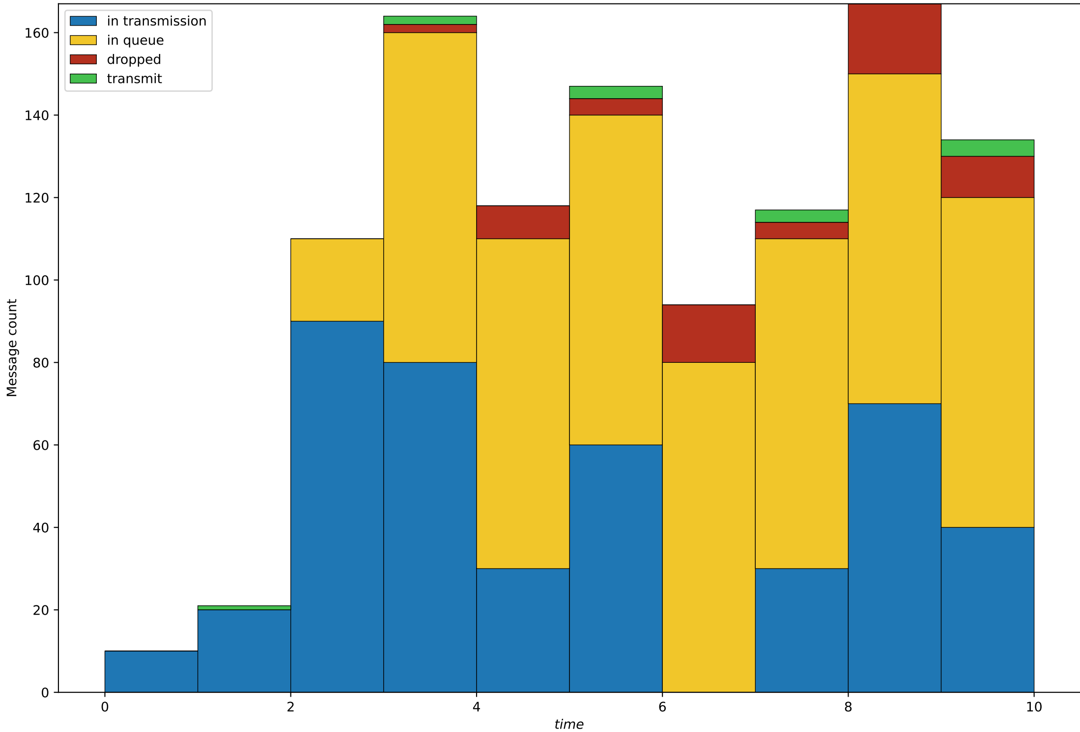
Duration=10, Clients count=1, Client's \lambda=6 , Servers count=1, Q=8
