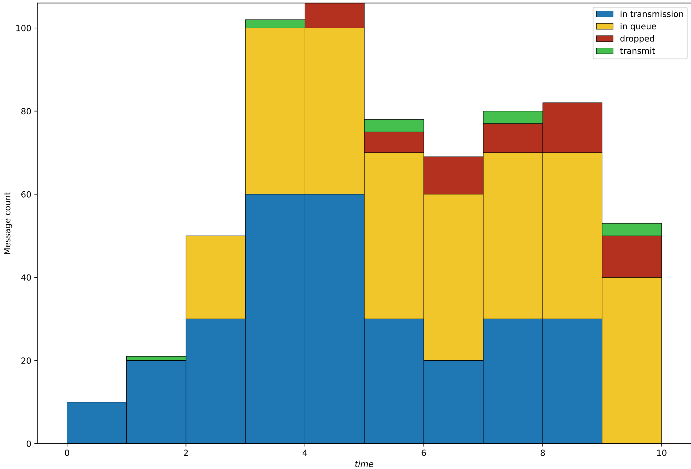
Duration=10, Clients count=1, Client's \lambda=4 , Servers count=1, Q=4
