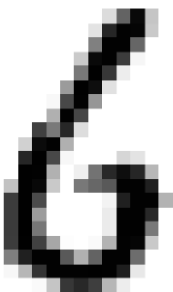
Label: 6
