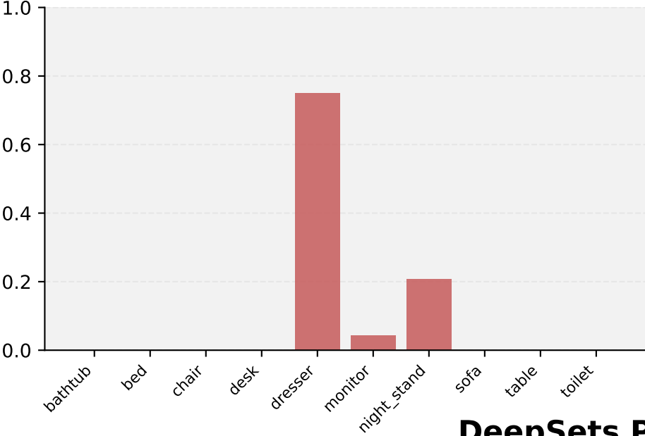
DeepSets Predictions
