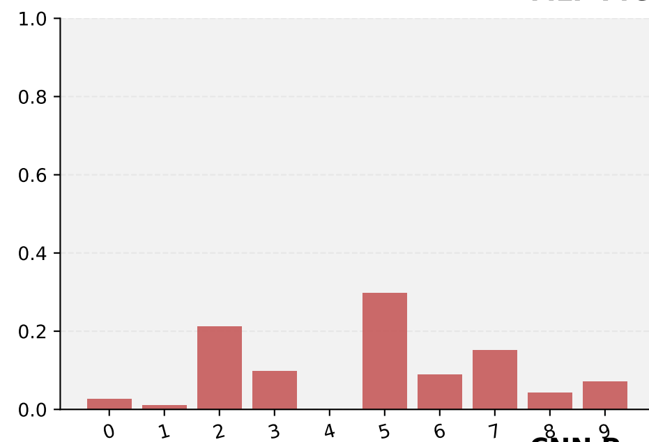
CNN Predictions
