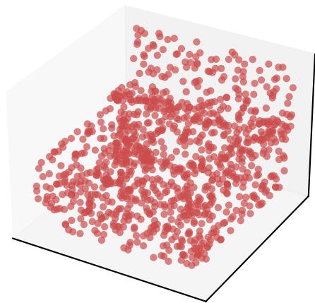
Label: bed
