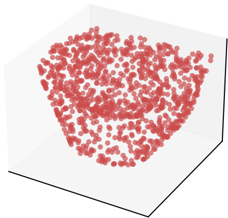
Label: toilet
