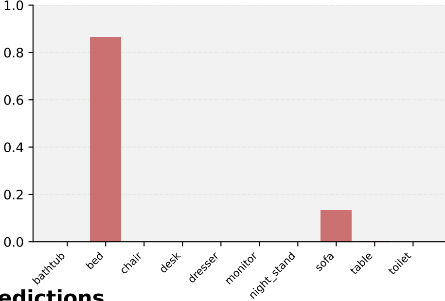
DeepSet Predictions
