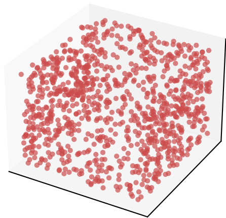
Label: dresser
