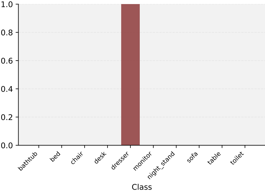
DeepSets Predictions
