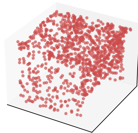
Label: desk
