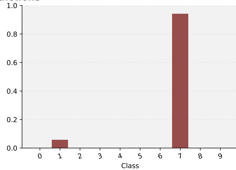
CNN Predictions
