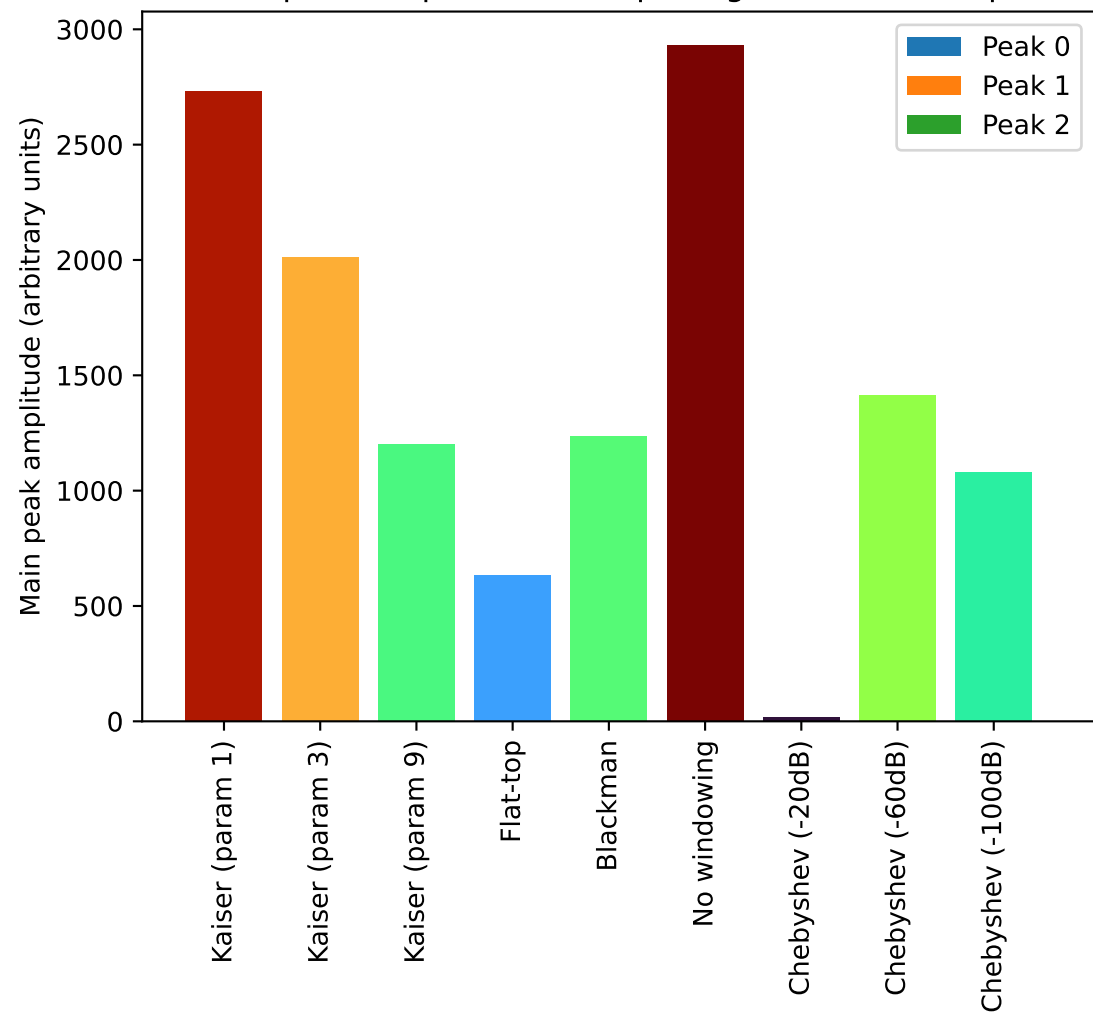
Main peak amplitude of output signal at 9.2 Hz input
