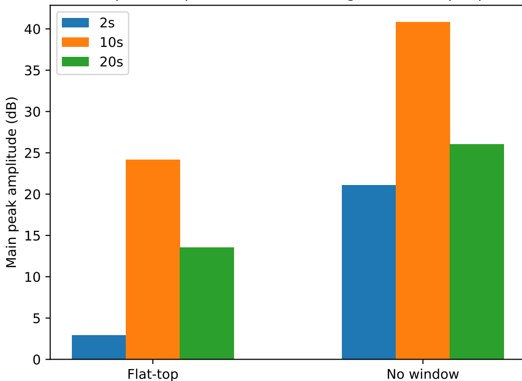
Main peak amplitude of transfer signal at sweep input
