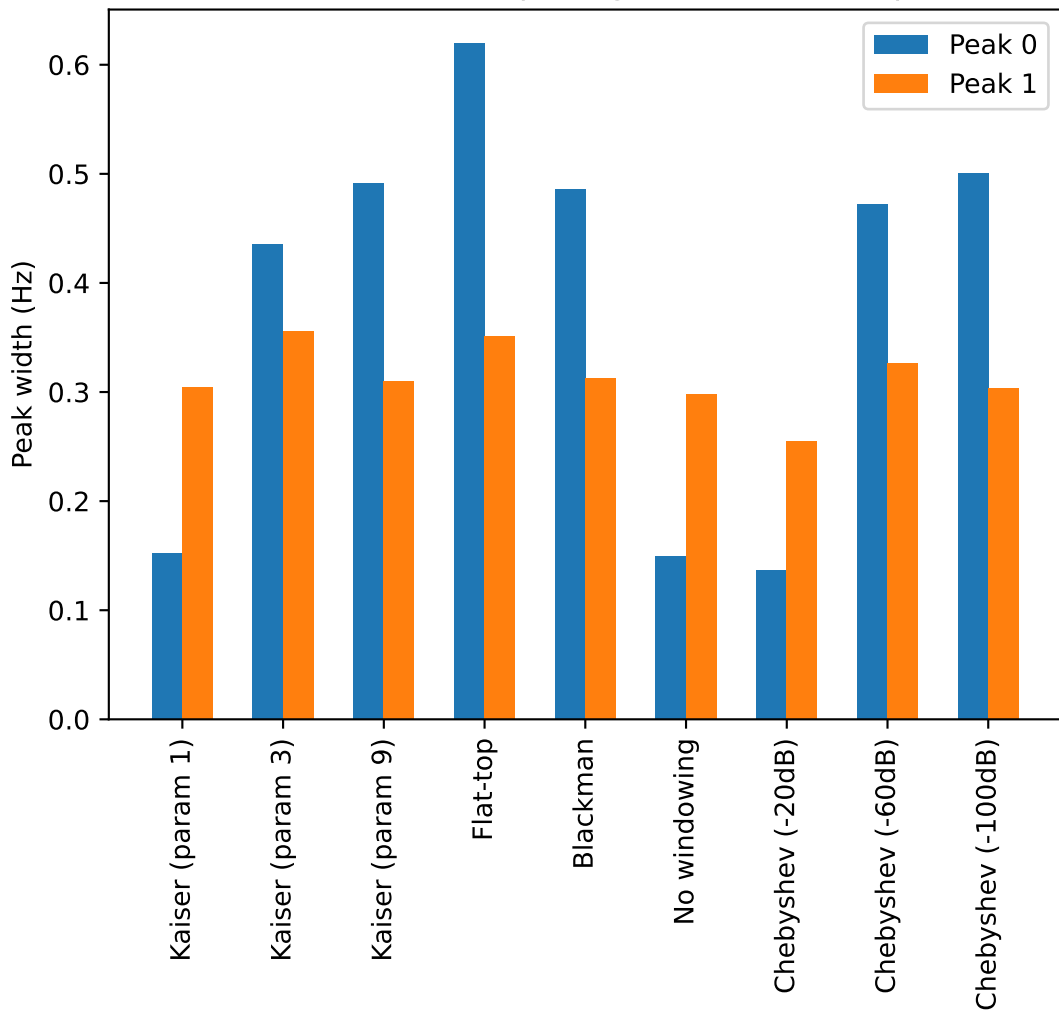
Peak widths of output signal at random input
