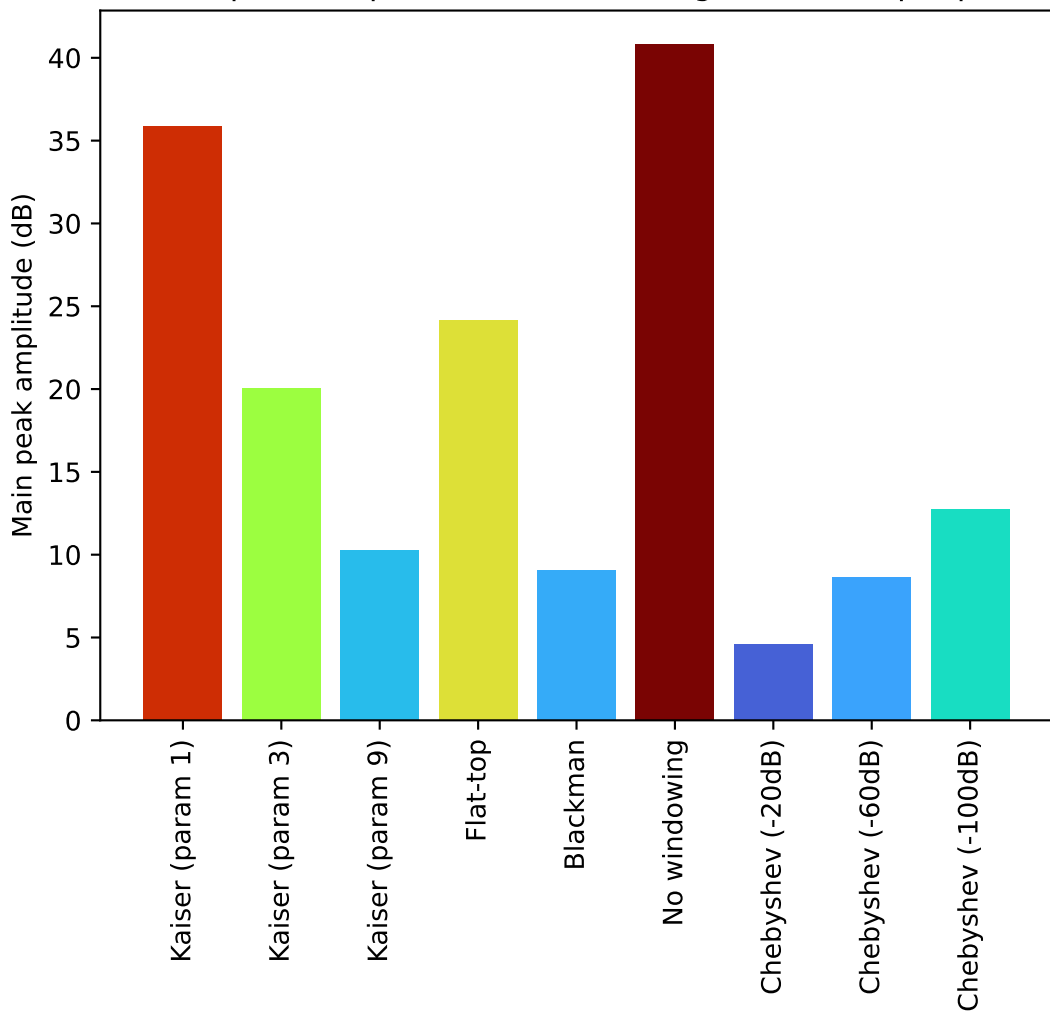
Main peak amplitude of transfer signal at sweep input
