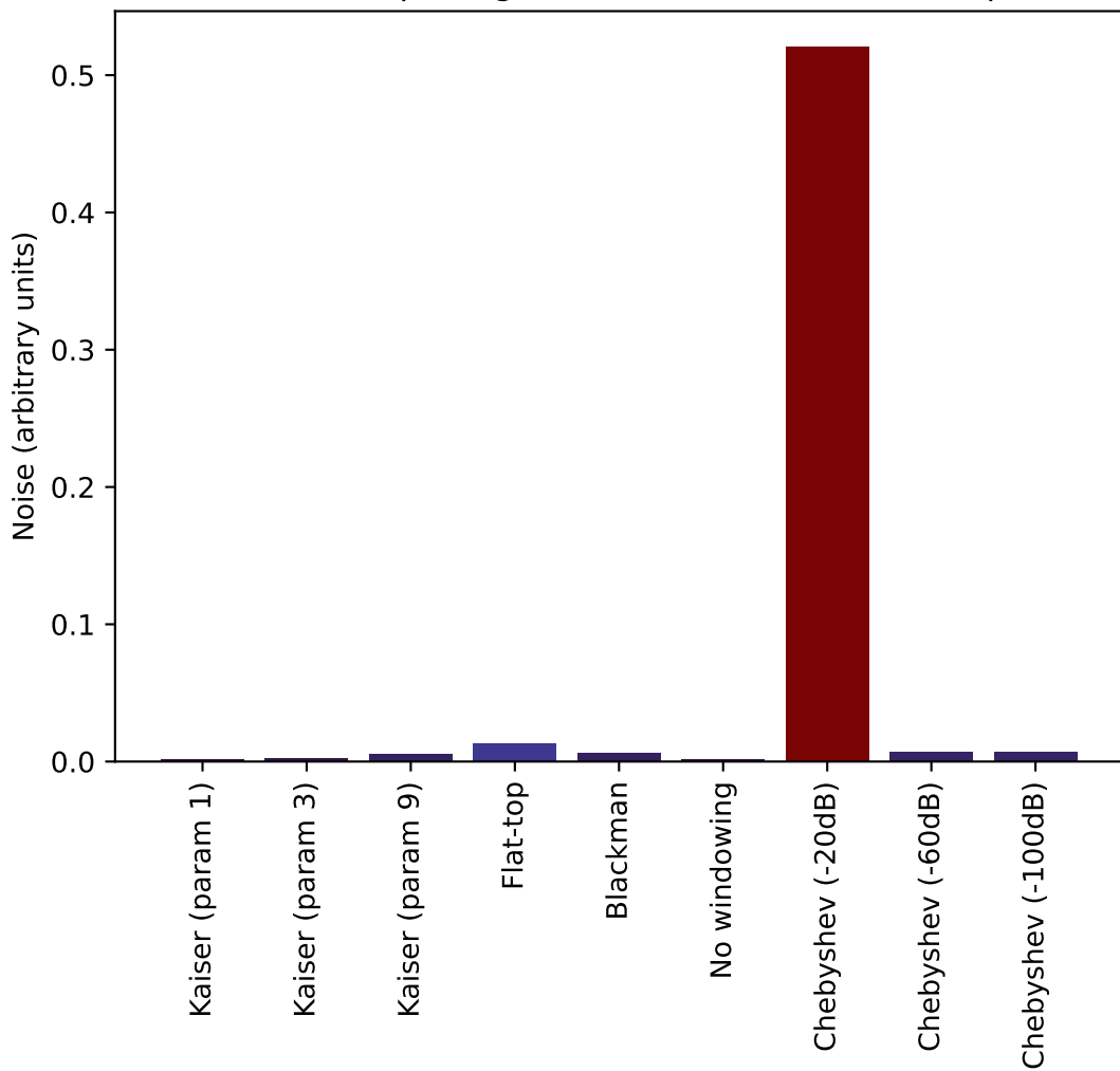
Noise of output signal at 9.2 Hz and 13.6 Hz input
