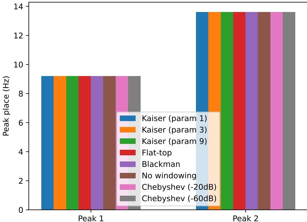
Peaks of output at 2x resonance input
