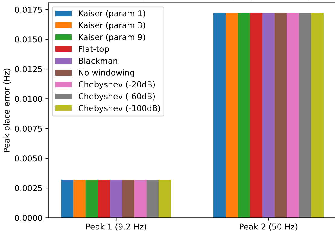
Error between input transform and programmed input
