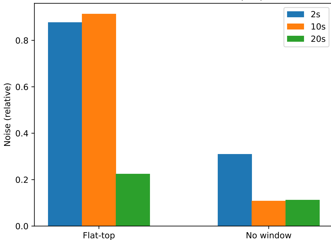
Noise of transfer at sine sweep input
