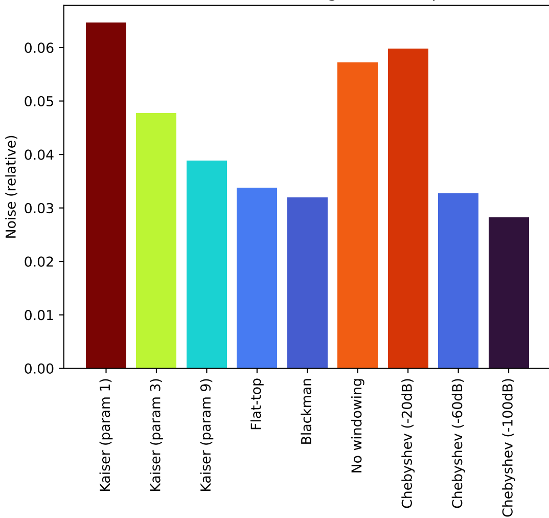
Noise of transfer signal at sweep
