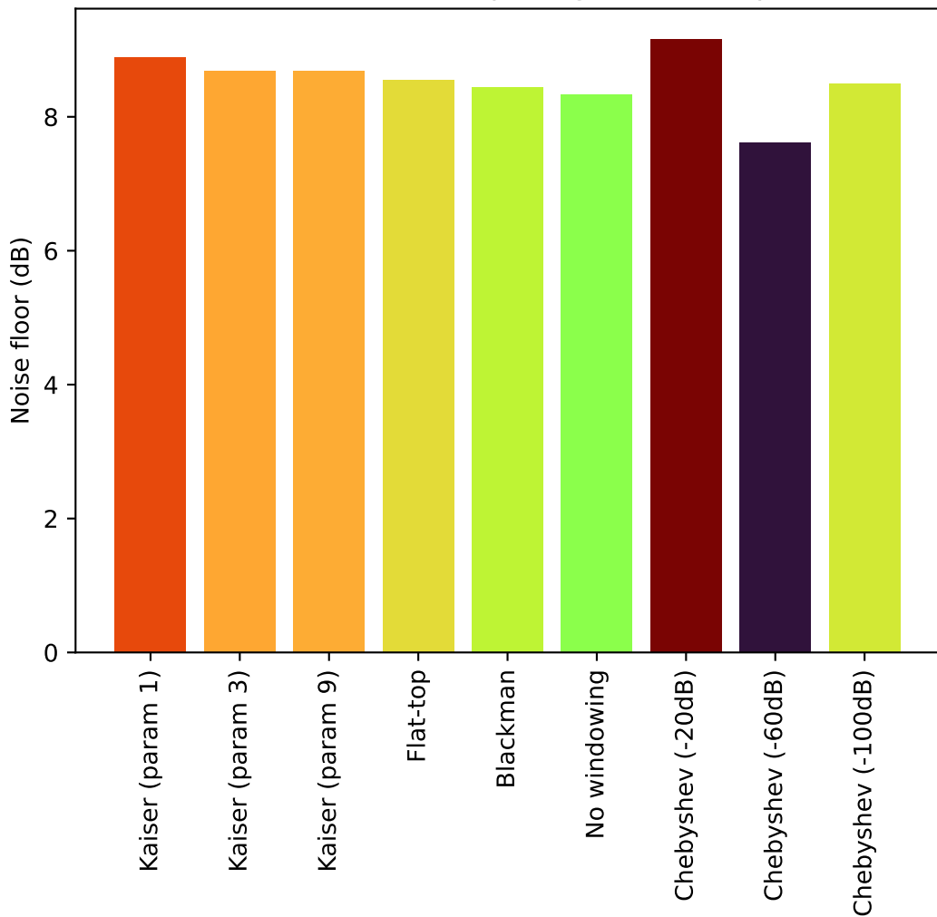
Noise floor of output signal at sweep
