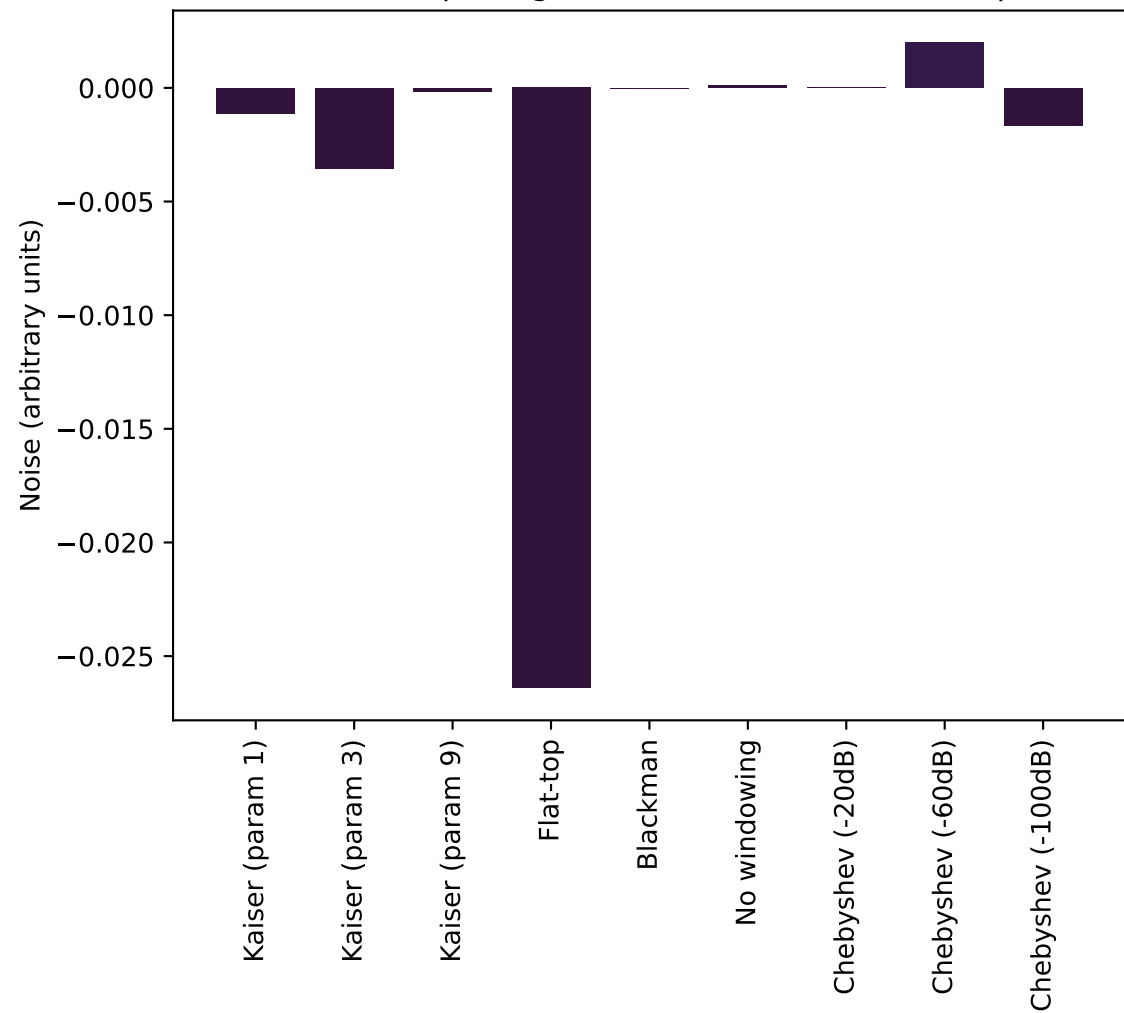
Noise of output signal at 9.2 Hz and 13.6 Hz input
