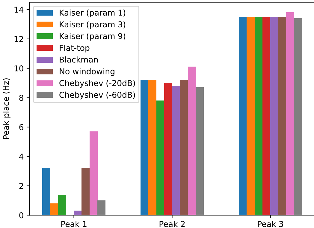
Largest 3 peaks of transfer at sweep input
