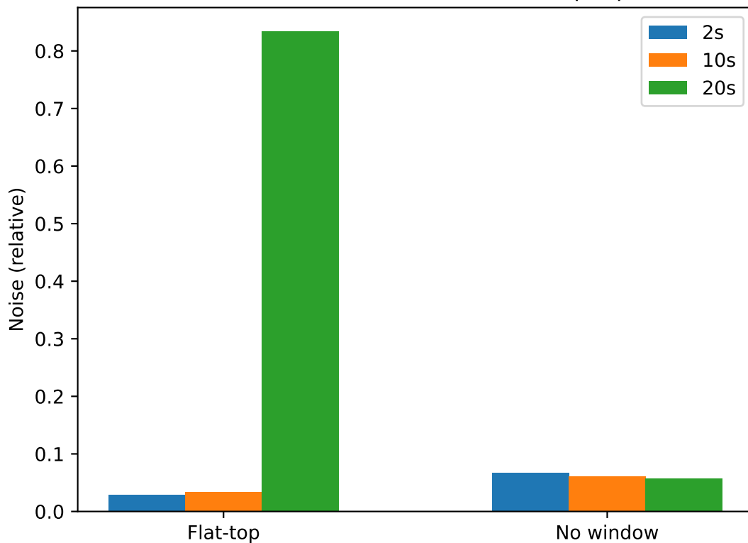
Noise floor of transfer at sine sweep input
