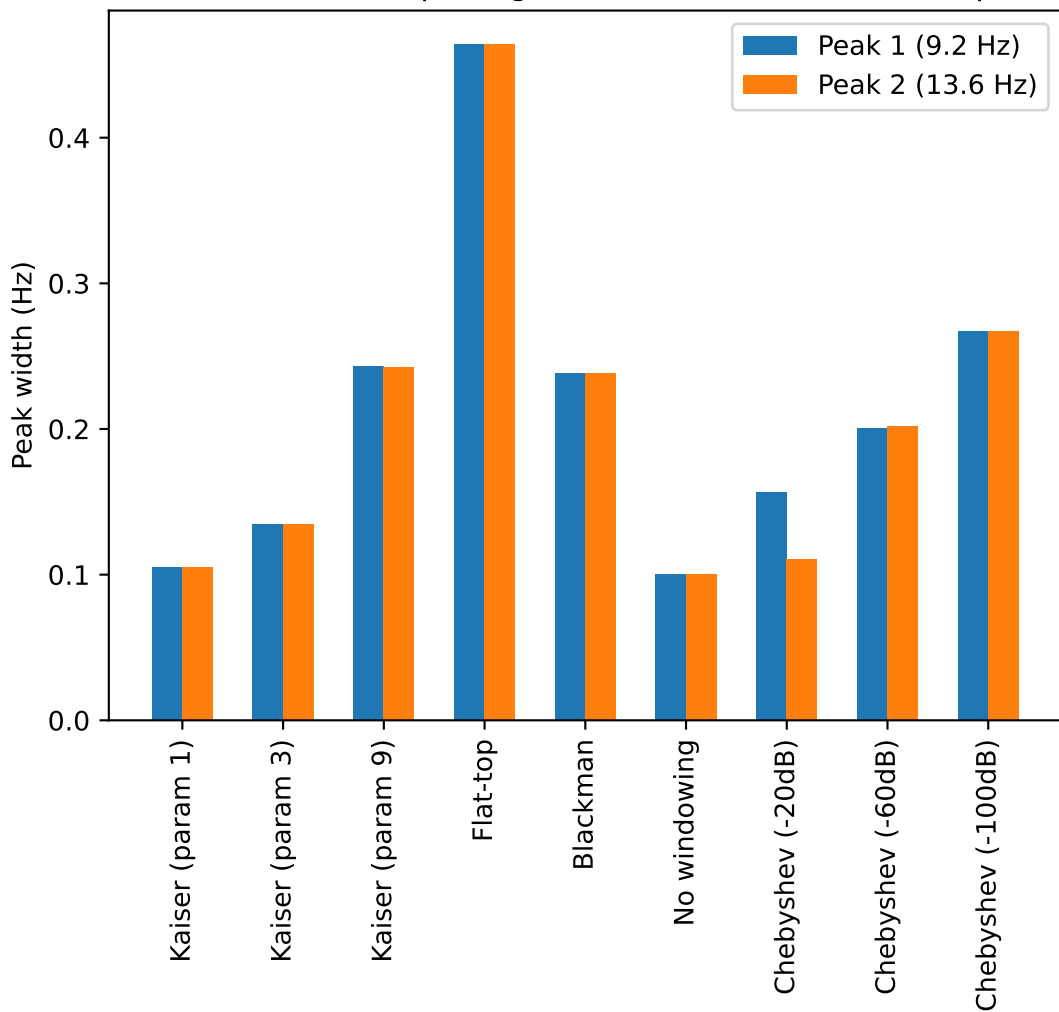
Peak width of output signal at 9.2 Hz and 13.6 Hz input
