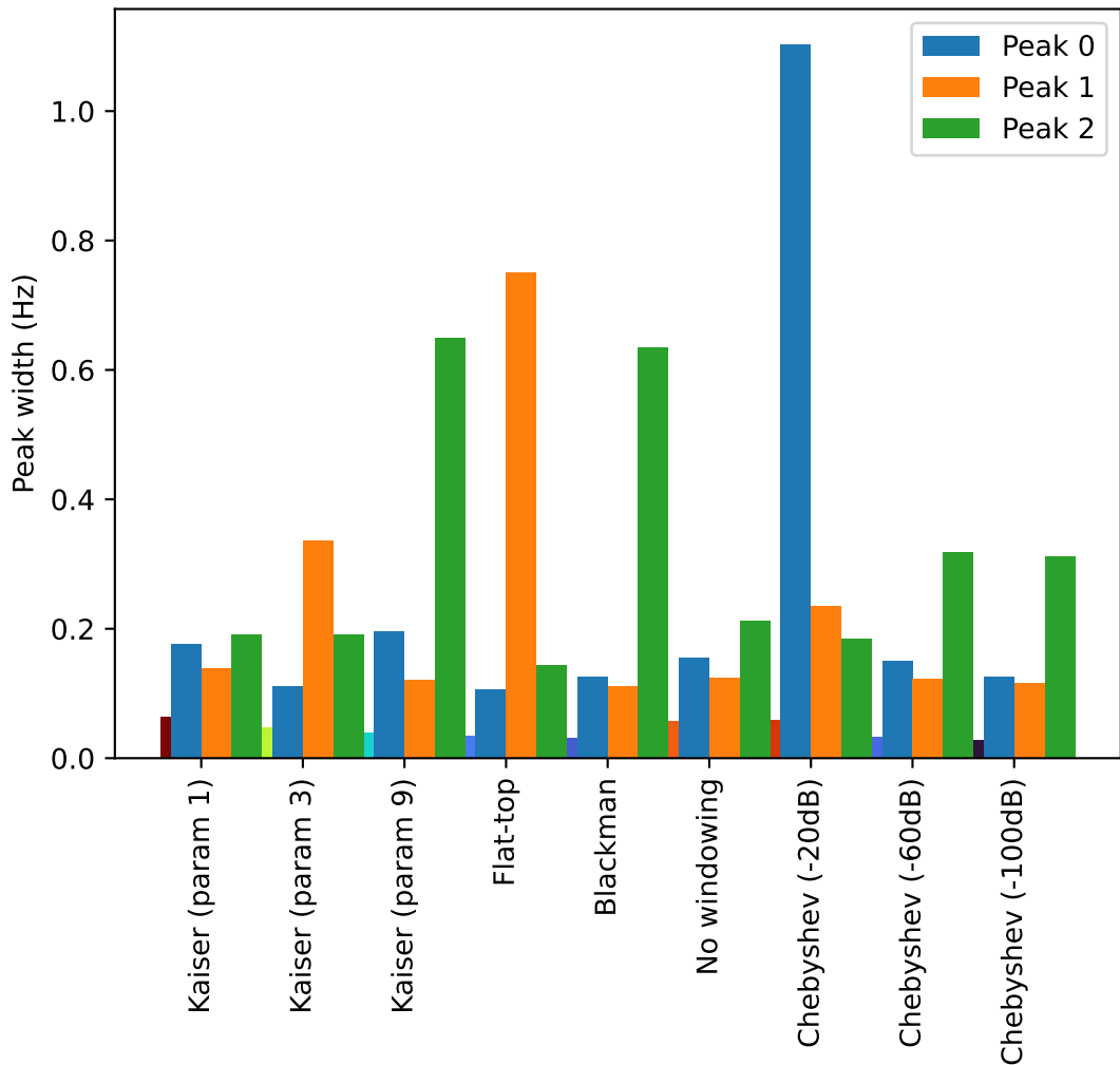
Peak width of transfer at sweep input
