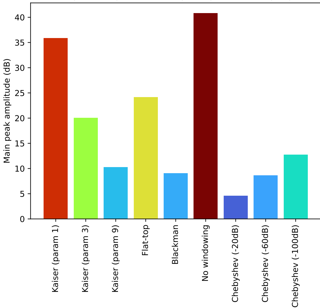
Main peak amplitude of output signal at sweep input
