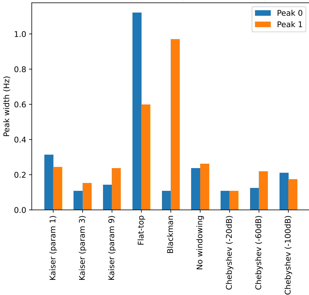
Peak widths of transfer signal at random input
