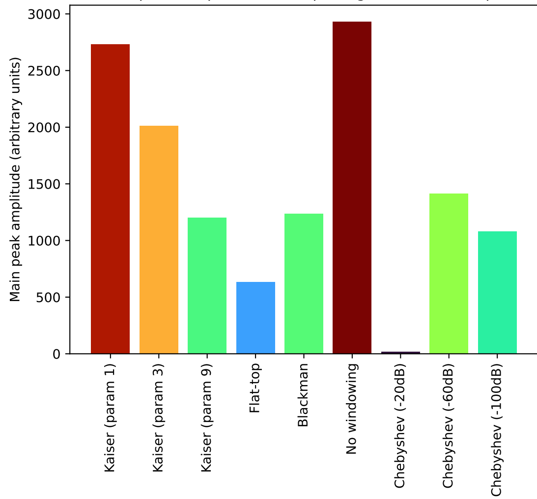
Main peak amplitude of output signal at 9.2 Hz input
