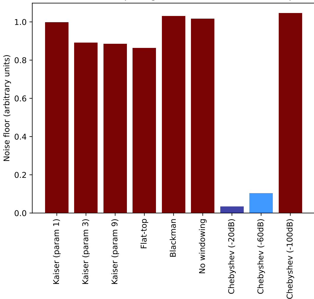
Noise floor of output signal at 9.2 Hz and 13.6 Hz input
