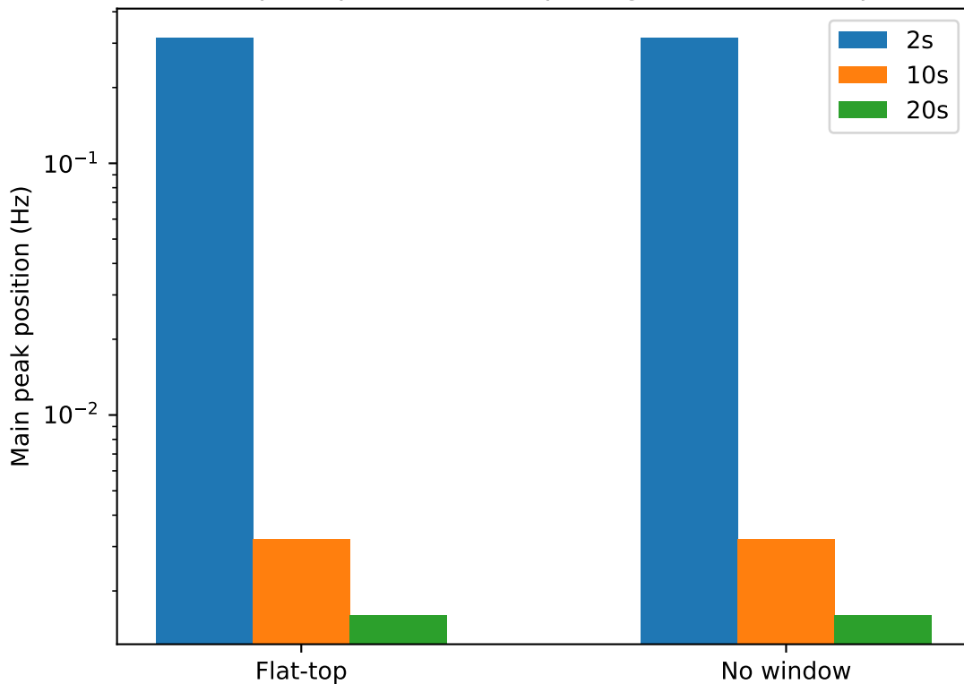
Main peak position of output signal at 9.2 Hz input
