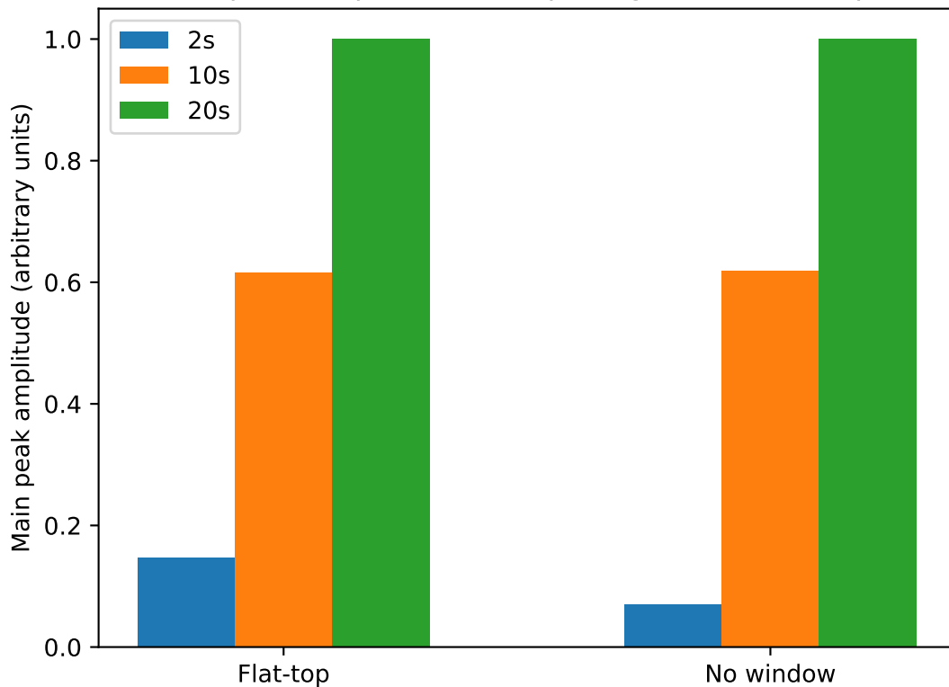
Main peak amplitude of output signal at 9.2Hz input
