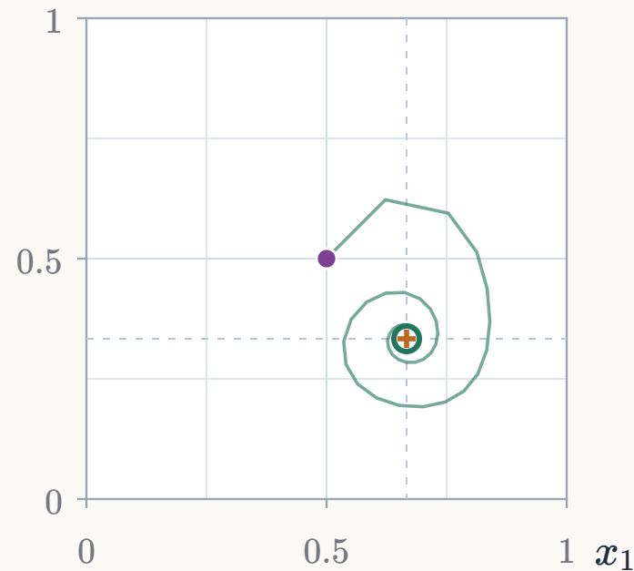
y_1 Optimistic MWU
