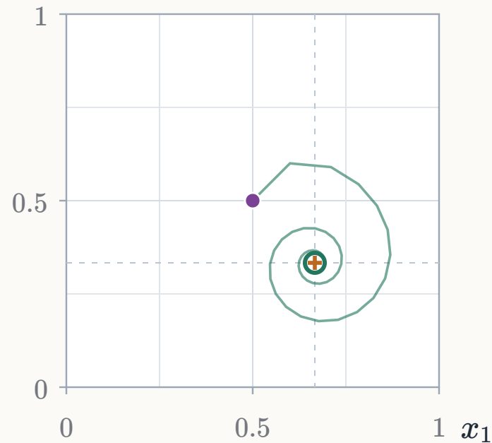
y_1 Optimistic OGD
