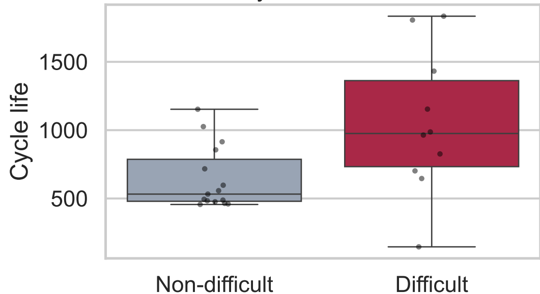
RUL: cycle-life distribution
