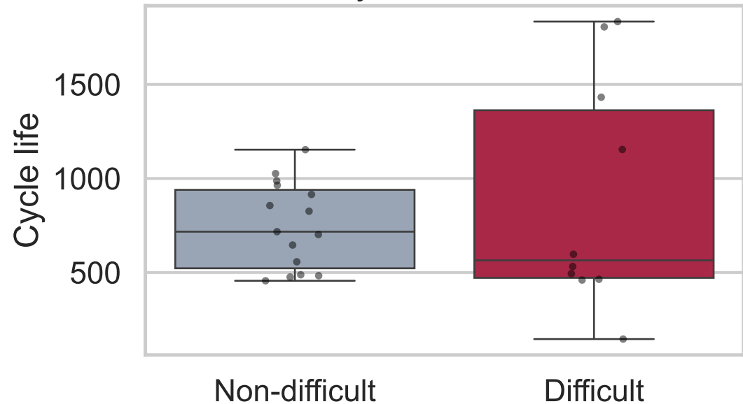
SOH: cycle-life distribution
