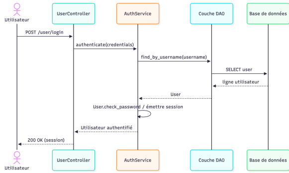
Figure A.8 : Authentification
