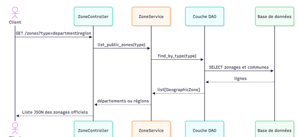
Figure A.7 : Zonages publics (F2)
