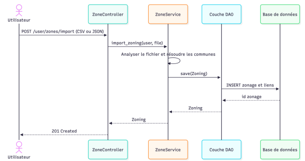
Figure A.11 : Import (FO3)
